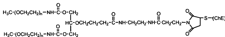
Example 1D Conjugate (each n defined to provide a ~30kDa PEG)
