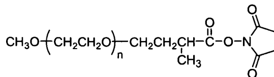
Linear mPEG-Succinimidyl \alpha -Methylbutanoate Derivative, 30kDa ("mPEG-SMB")
