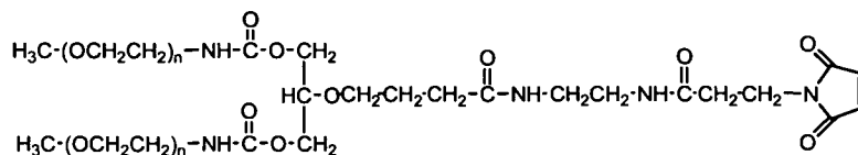
Branched 60kDa PEG Bearing a Maleimide Group (each n defined to provide a ~30kDa PEG)
