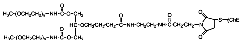
Example 1C Conjugate
