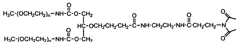
Branched 40kDa PEG Bearing a Maleimide Group
