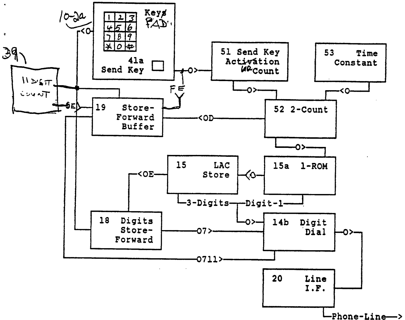
FIGURE 2a. Cellular, Dual Actuation of Send Key
