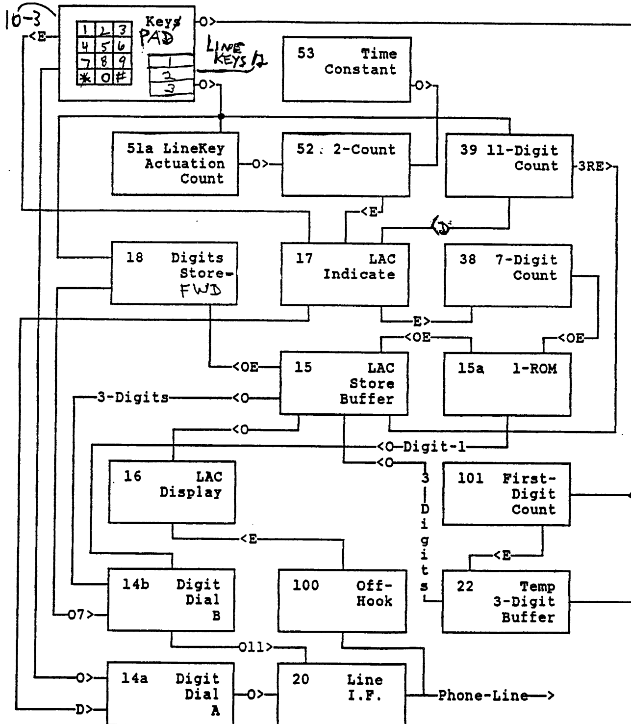
FIGURE 3. Keyphone with Store-Forward
