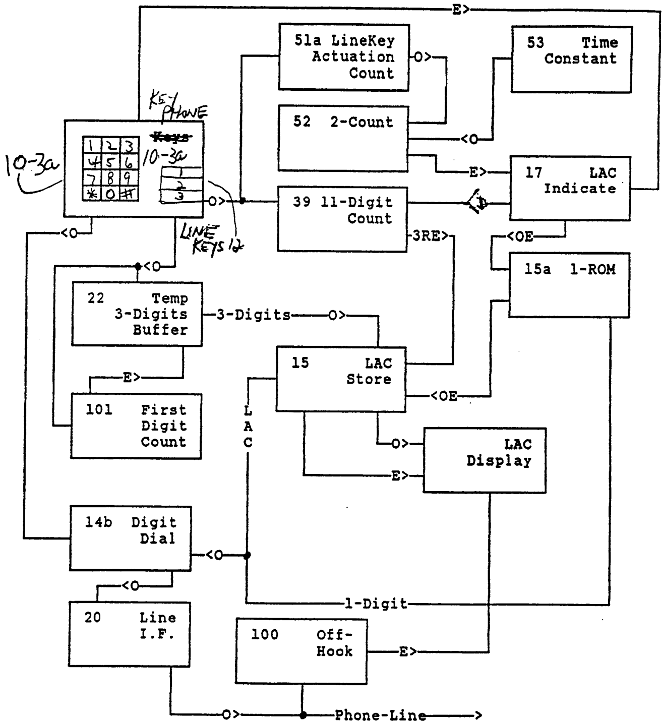
FIGURE 3a. Keyphone without Store-Forward
