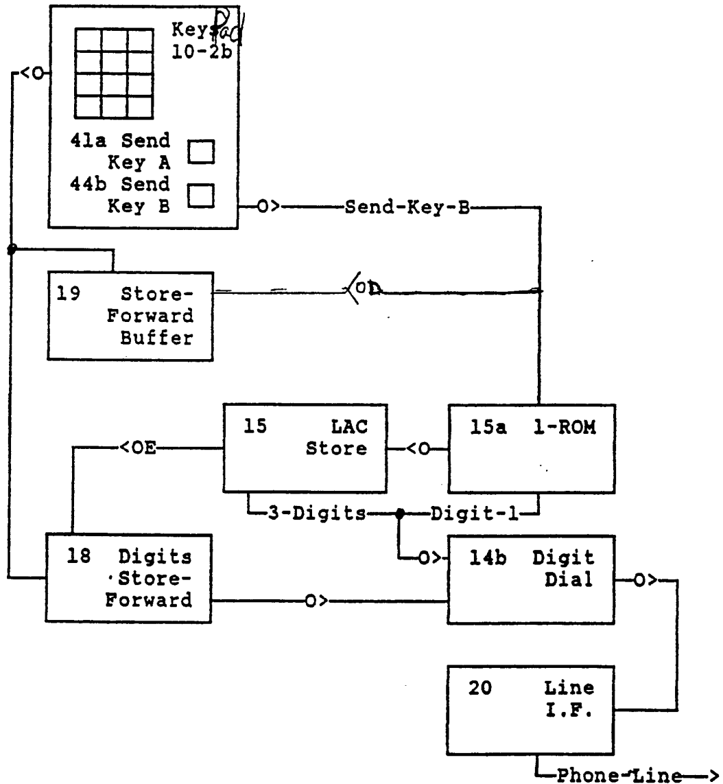
6 FIGURE 2b. Cellular, Two Send Keys
