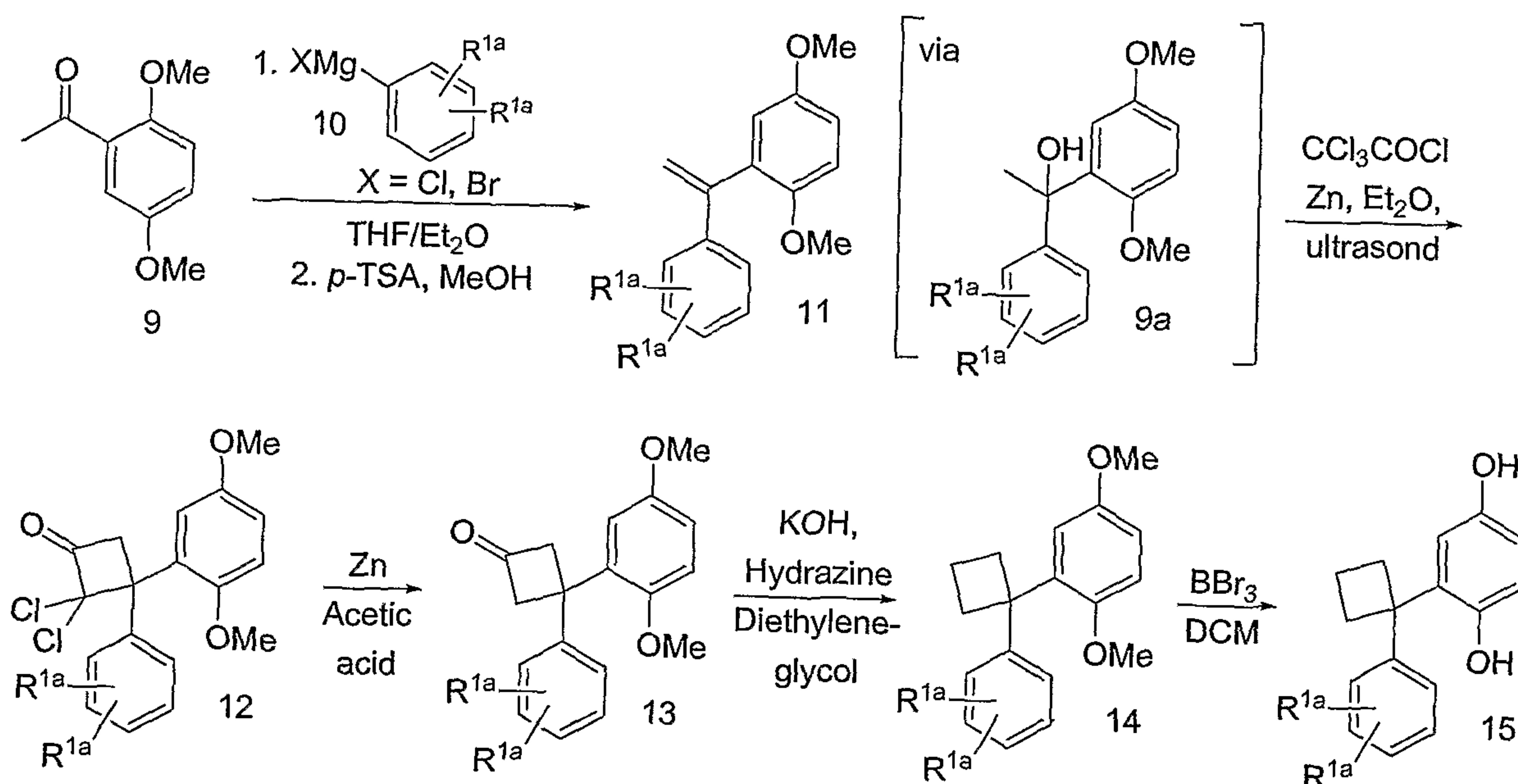
Scheme B
