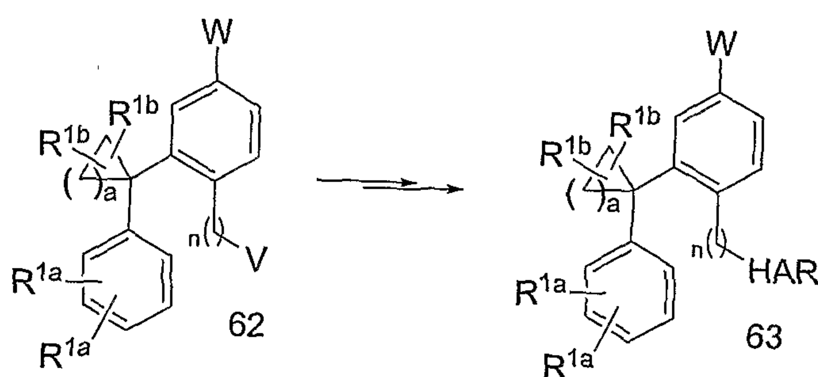
Scheme P
