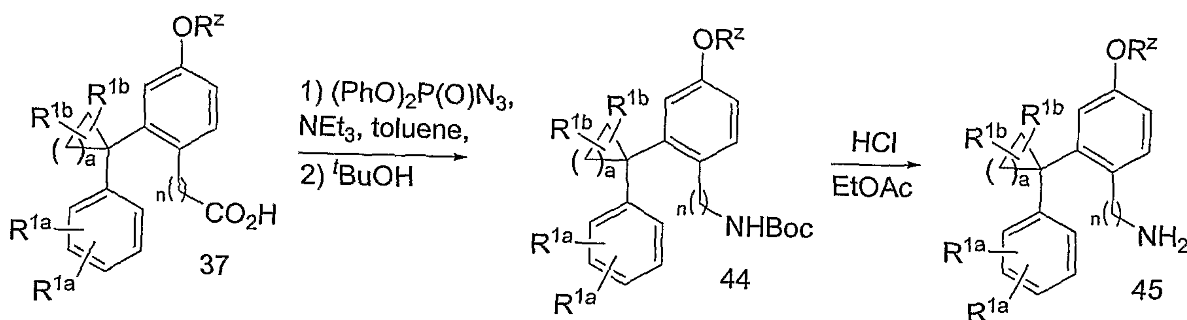
Scheme L
