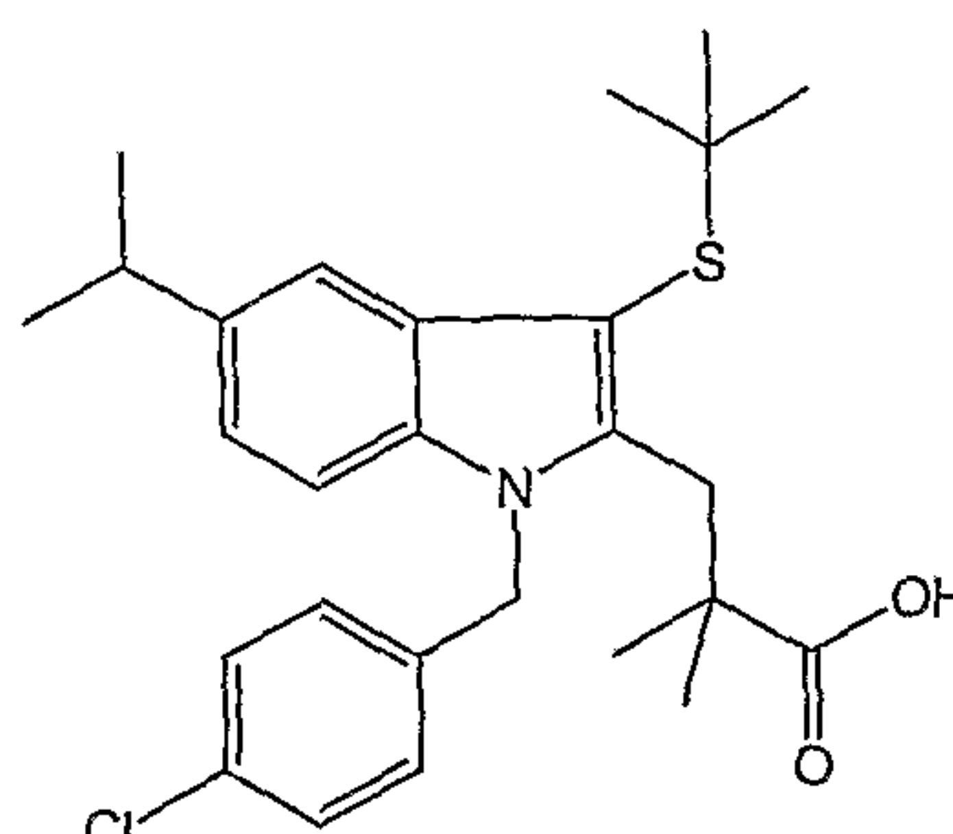
Compound B
