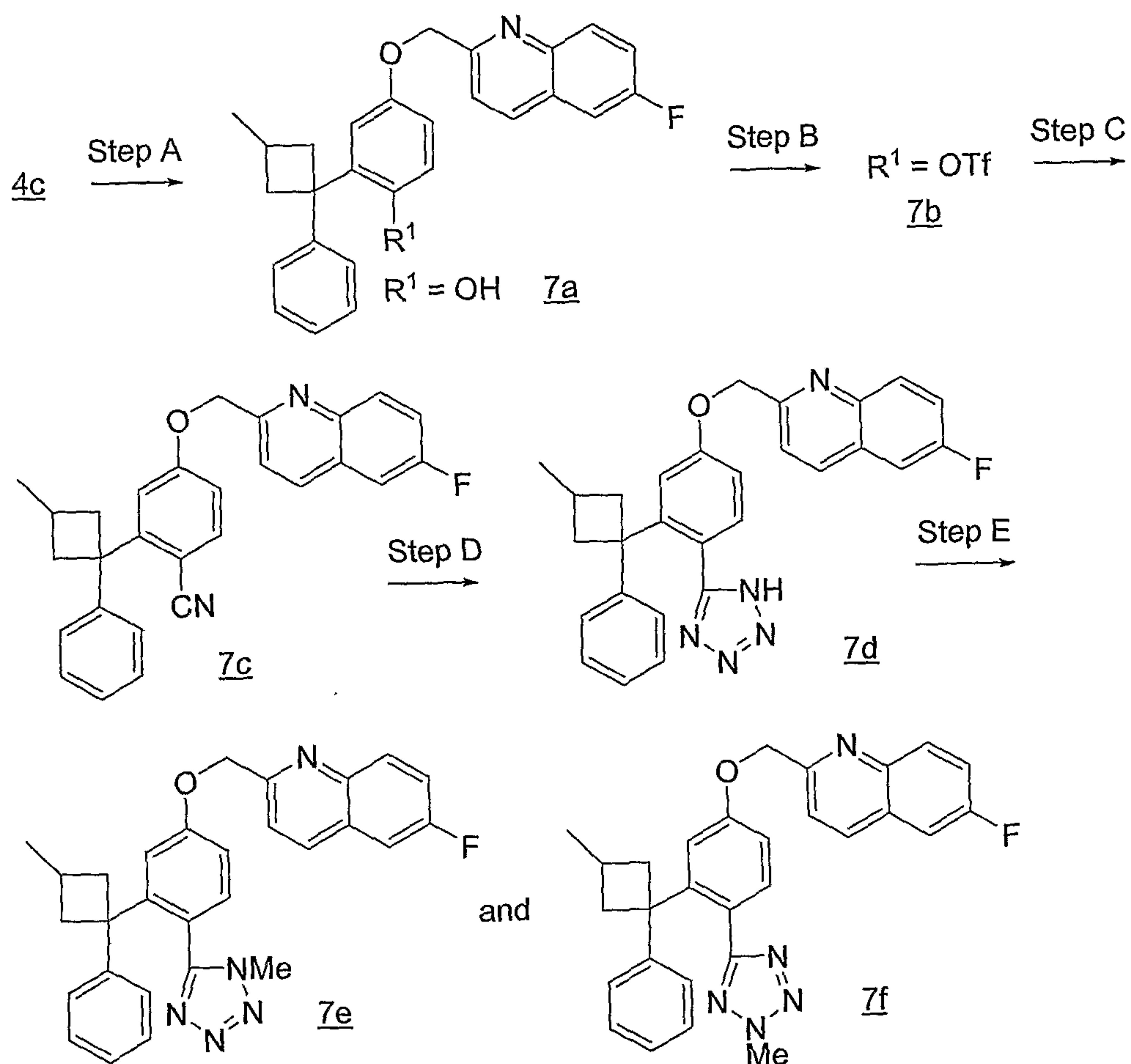
Scheme 7
