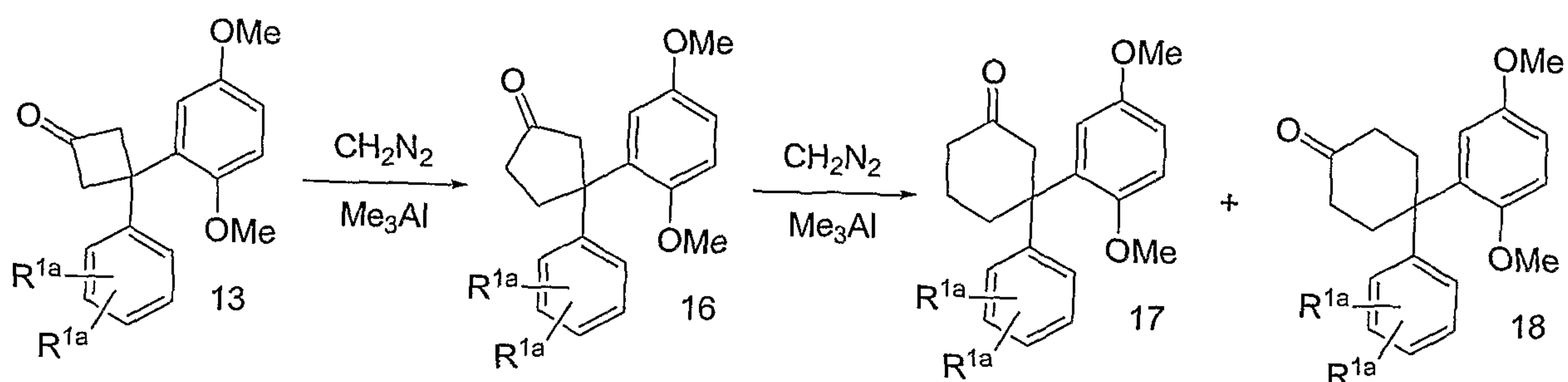
Scheme C
