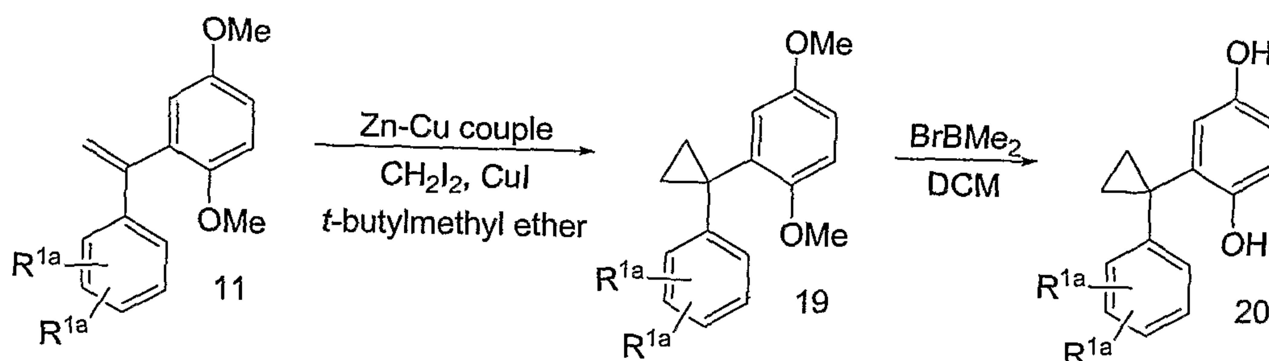
Scheme D
