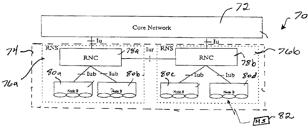
Fig. 4 (Prior Art)
