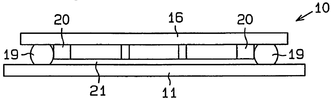
Fig.2 (Prior Art )
