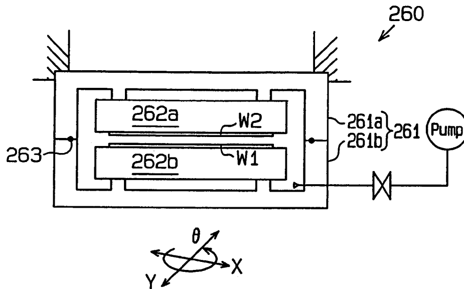
Fig.37 (Prior Art )
