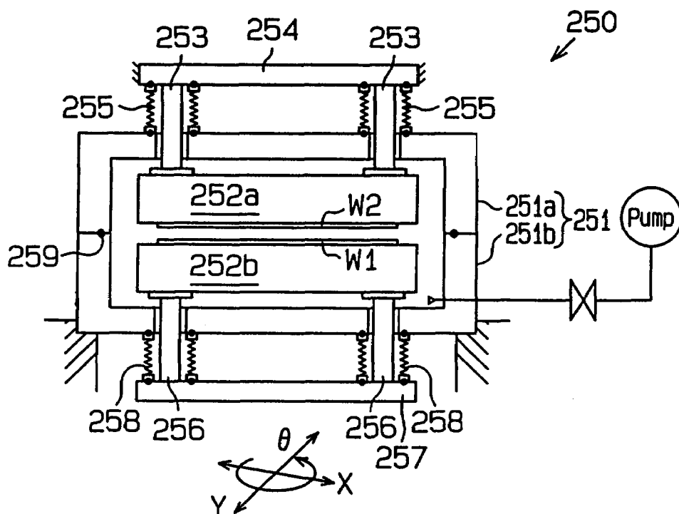
Fig. 36 (Prior Art)
