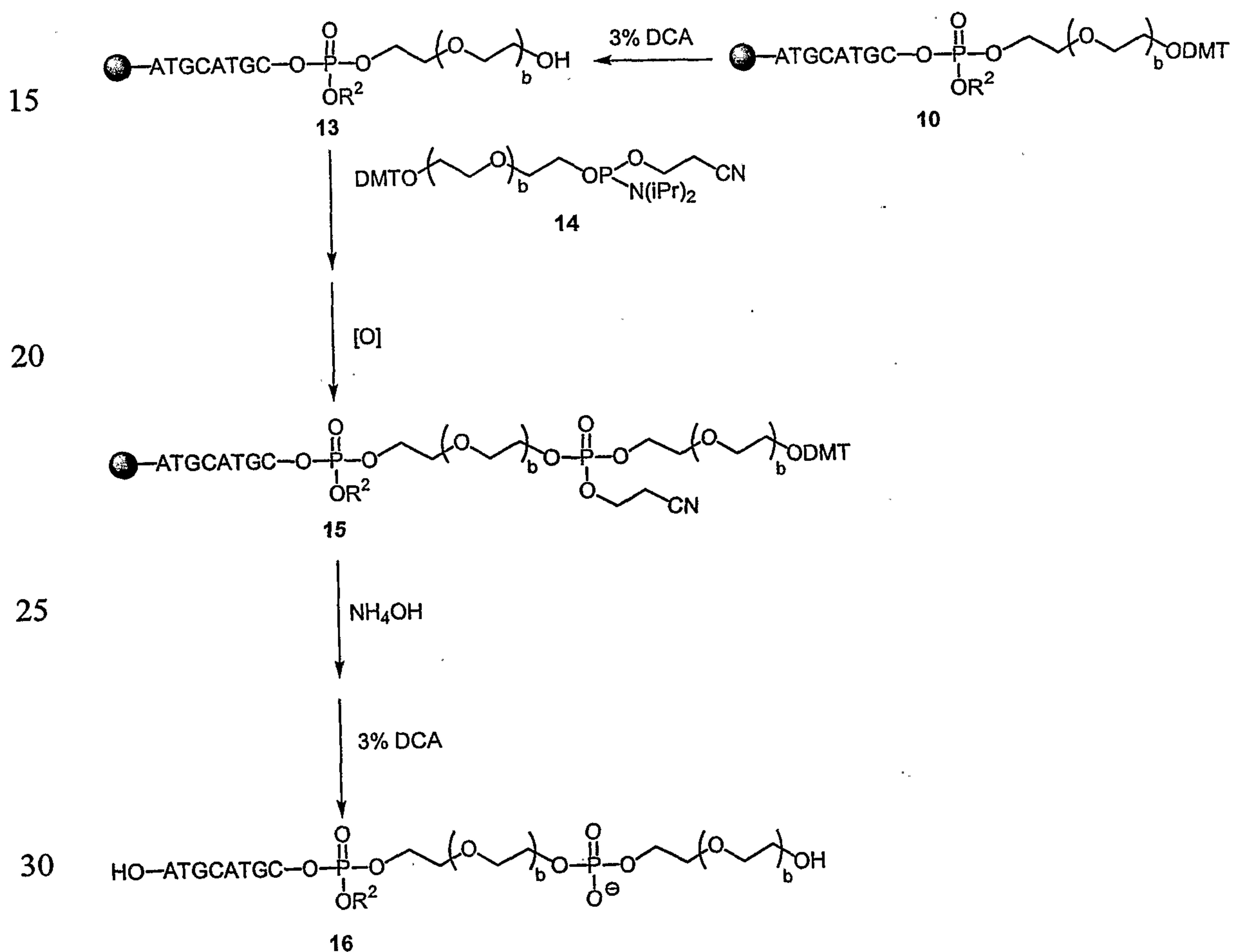
Scheme (III)
