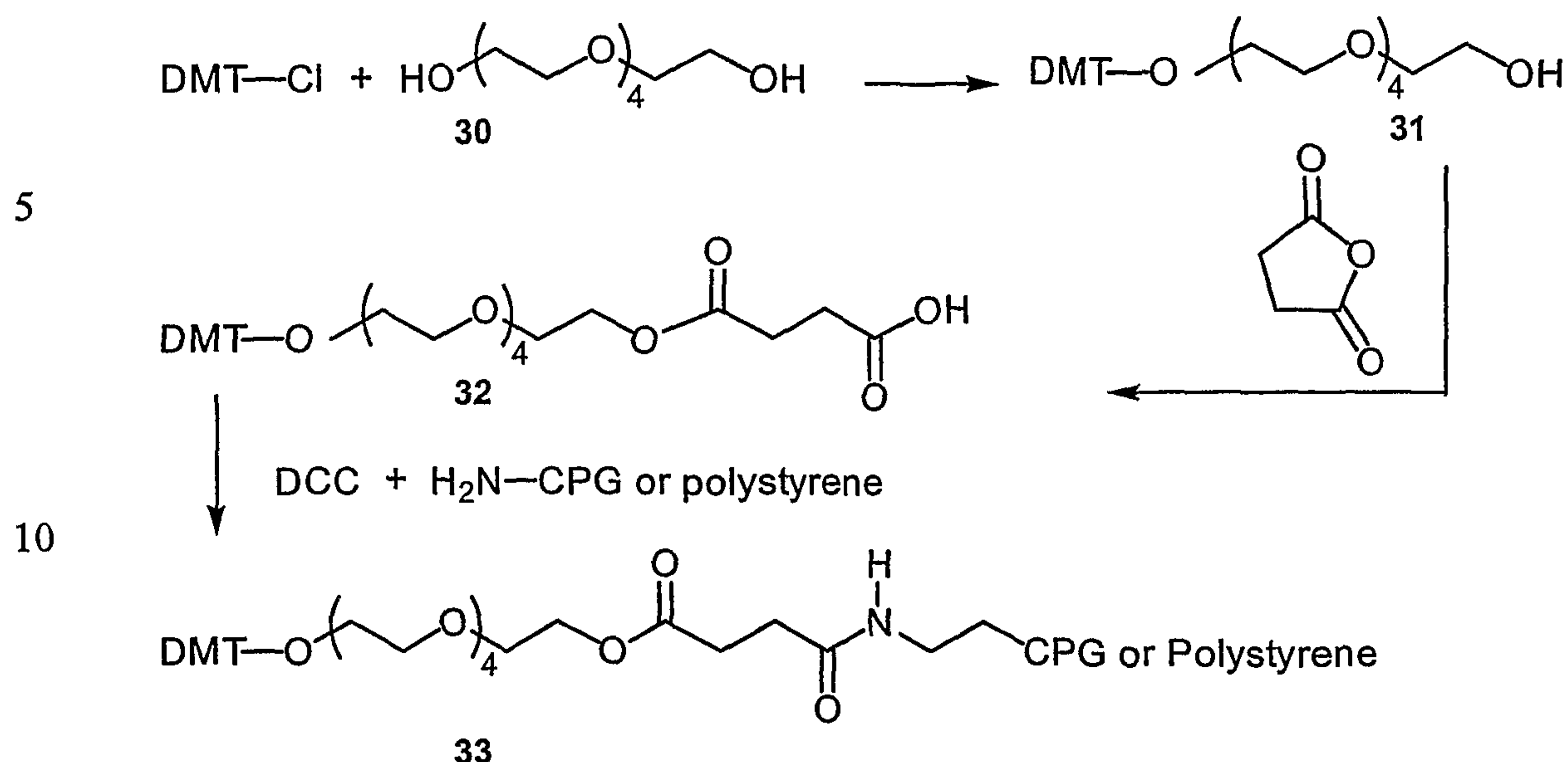
Scheme (VI)
