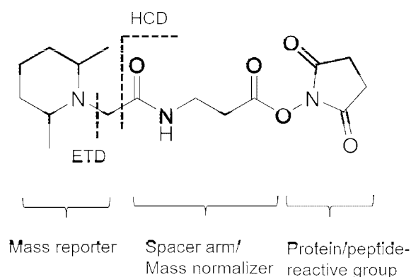
Scheme 1. Chemical structure of the tandem mass tag (TMT) reagent used in some aspects of the present disclosure.
