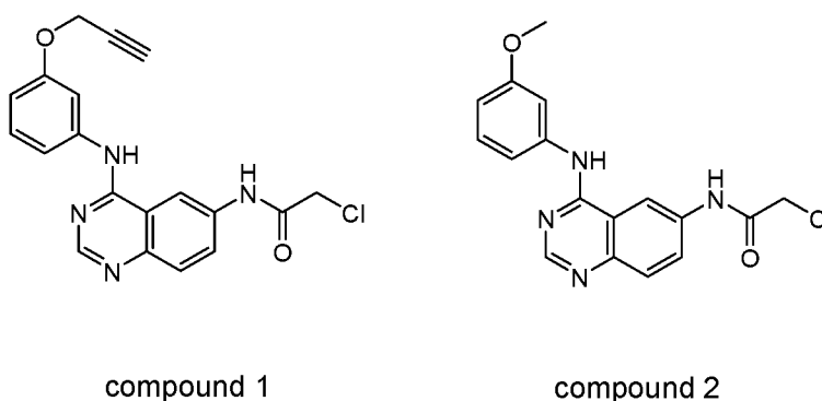
Scheme 2. Chemical structures of compound 1 and compound 2.
