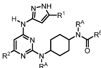
( Formula VIa )
