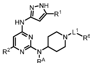
( Formula II )
