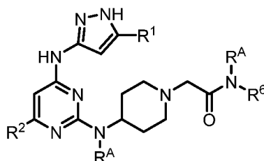
( Formula IIa )
