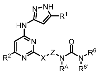
(Formula IIIa)
