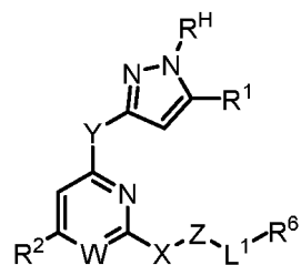
( Formula V )
