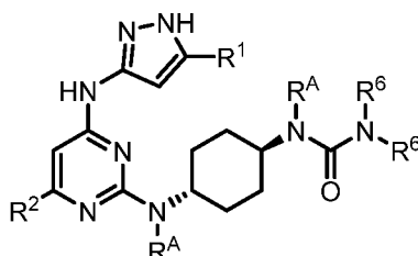
(Formula IVa)
