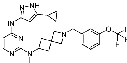
27
