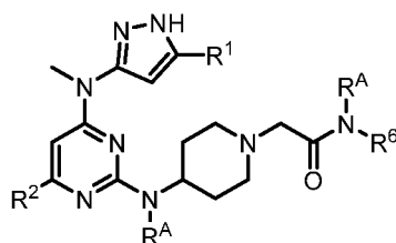
(Formula IIc)
