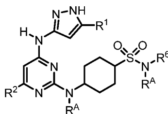
( Formula VIj )
