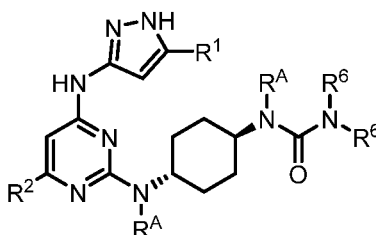
( Formula IVa )
