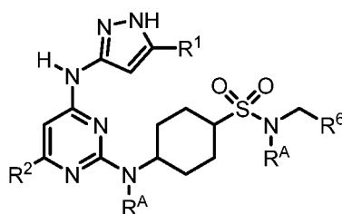
(Formula VII)
