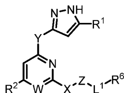
( Formula I-A )
