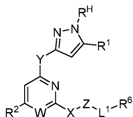
(Formula Iaa)
