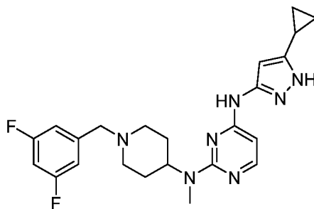
40
