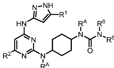
( Formula IV )
