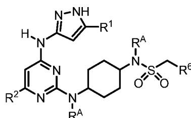
( Formula VIi )
