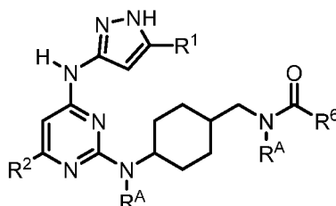
( Formula VIb )
