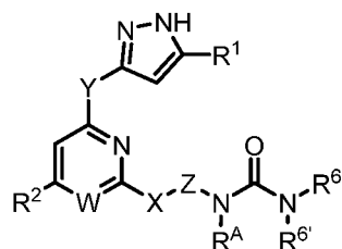
(Formula III-A)
