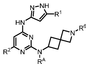
(Formula IId)
