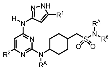
( Formula VIk )
