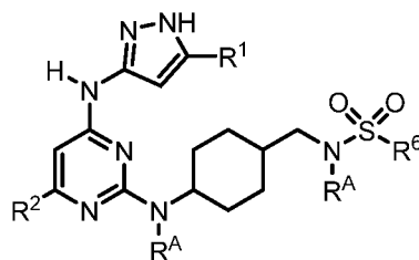
( Formula VIh )
