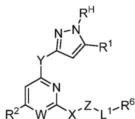
(Formula I)
