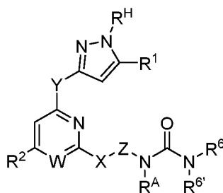
(Formula III)
