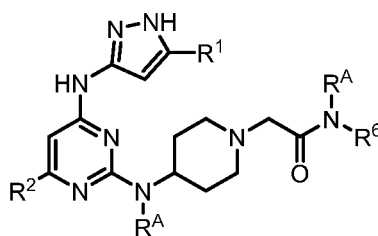
(Formula IIa)
