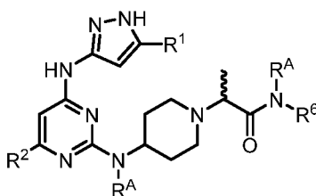
(Formula IIb)
