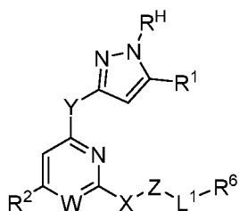
(Formula Iaa)
