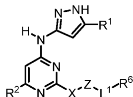
(Formula Va)
