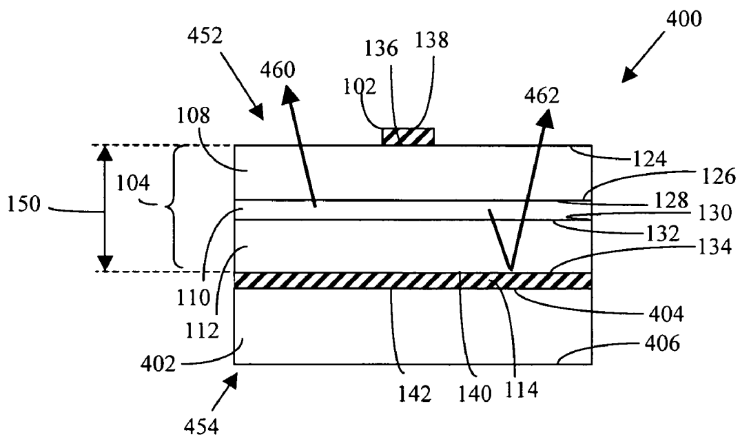
PRIOR ART FIG. 4B
