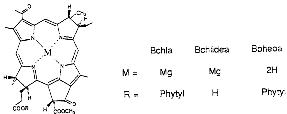
b) Structure of Bacteriochlorophyll a
