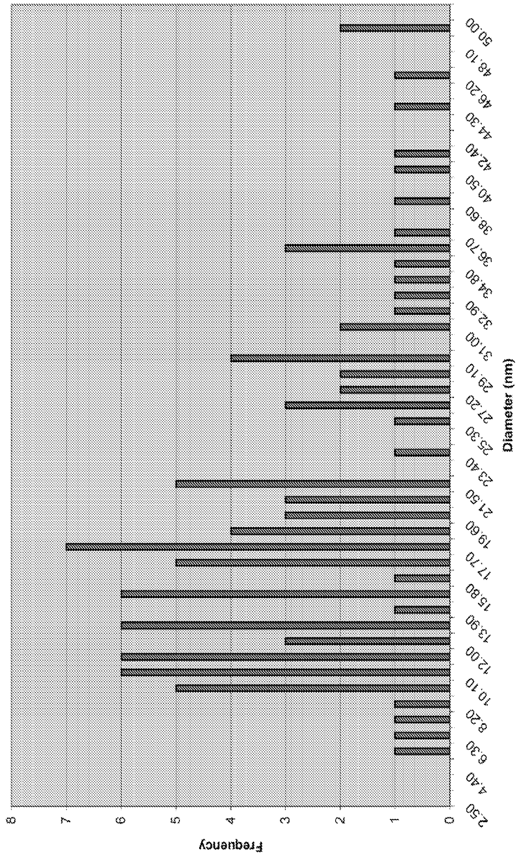
Figure 49b GB-020 TEM Size Distribution
