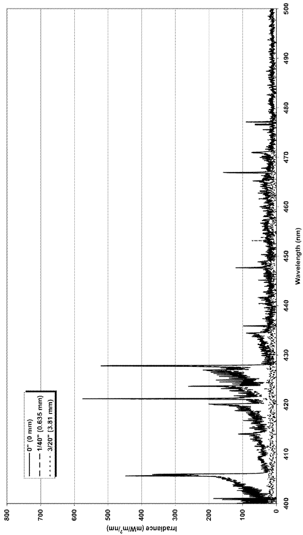
Figure 81 c. Ag Electrode Plasma Irradiance
