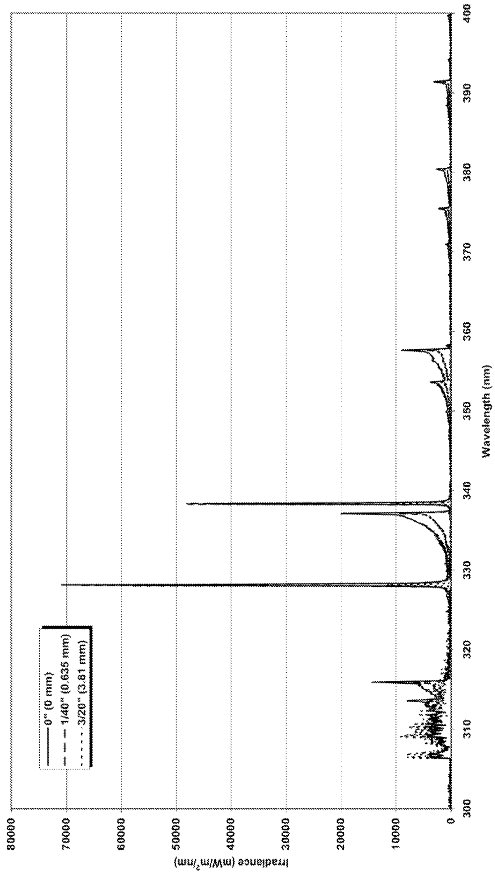
Figure 81 b. Ag Electrode Plasma Irradiance
