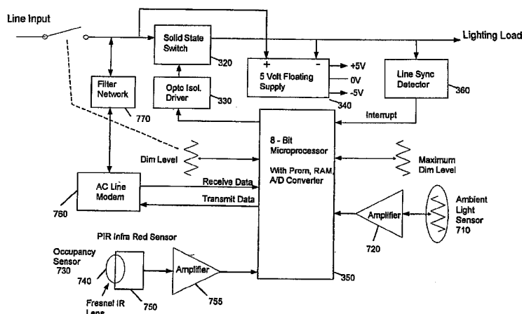
UCD-2 Block Diagram
