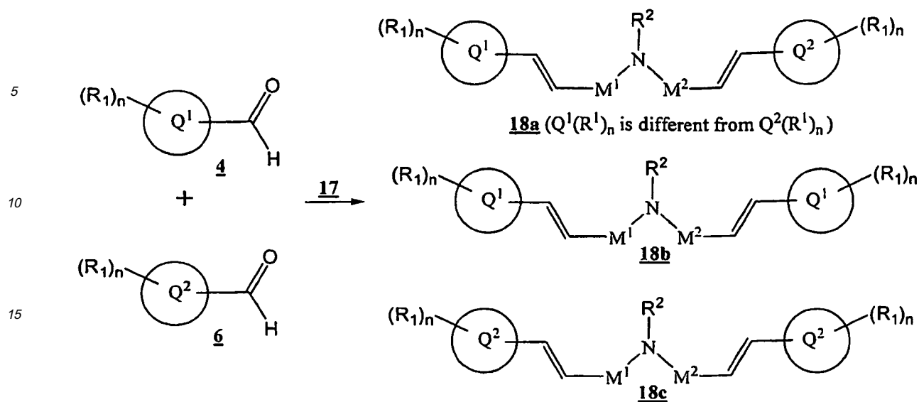
Scheme 13
