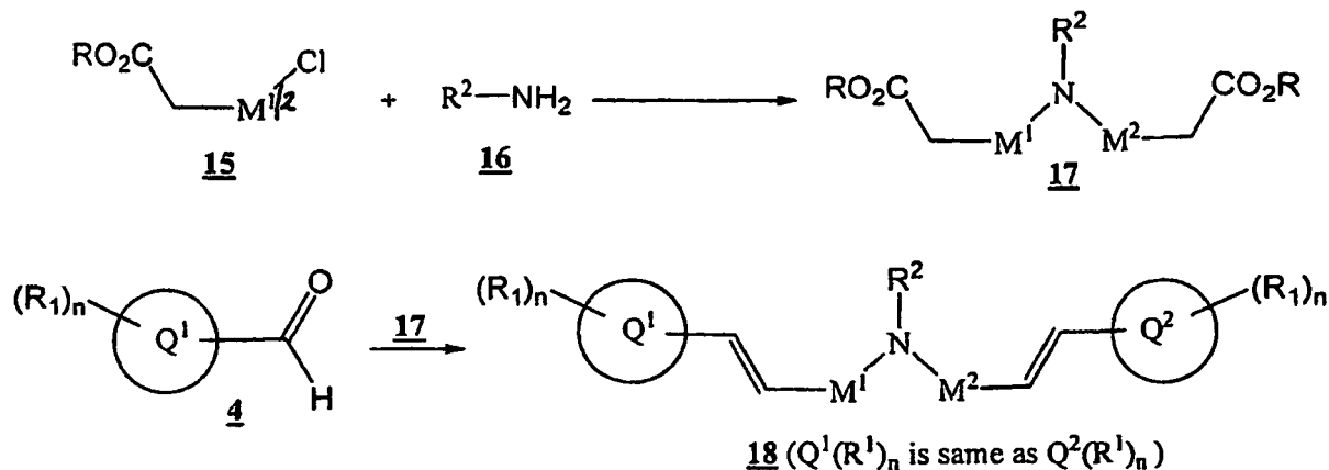
Scheme 12
