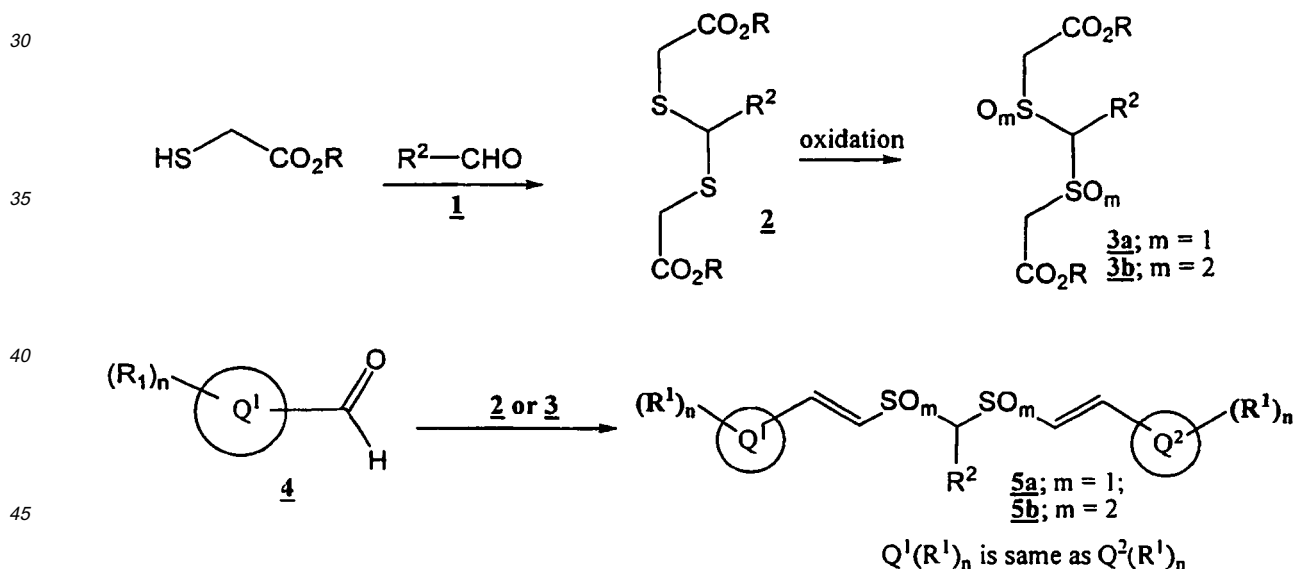
Scheme 7
