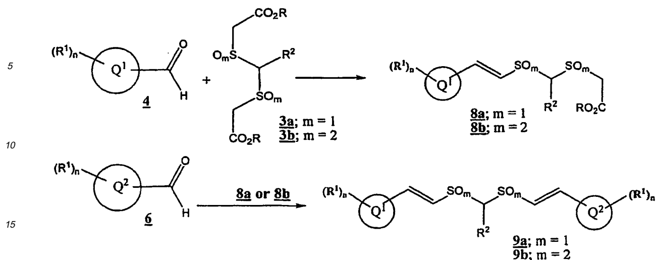
Scheme 9
