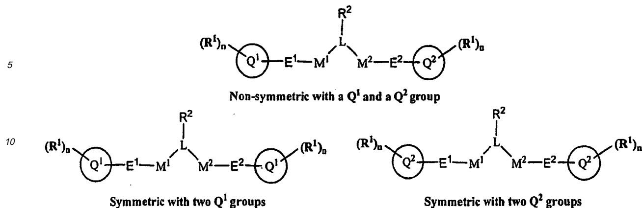
Scheme 6
