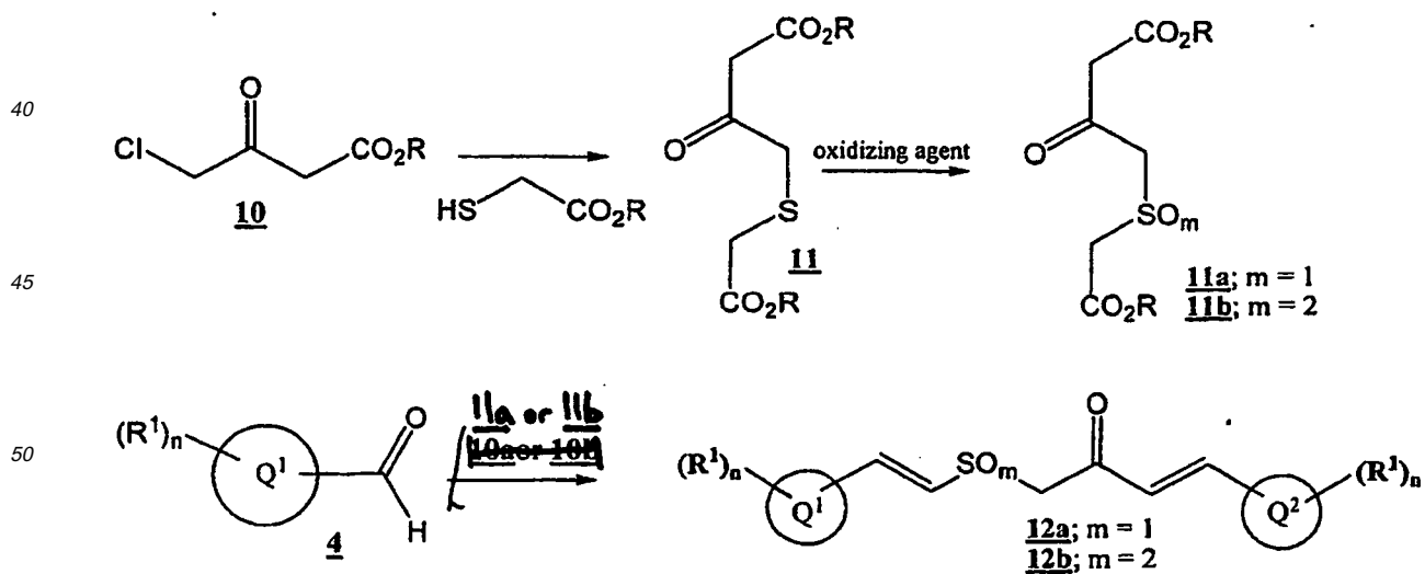
Scheme 10
