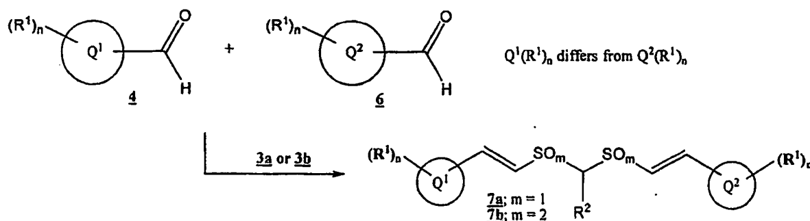
Scheme 8
