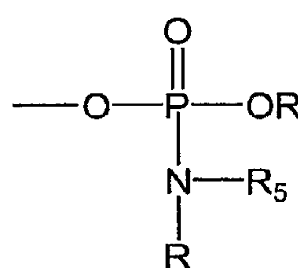
phosphoramidate
