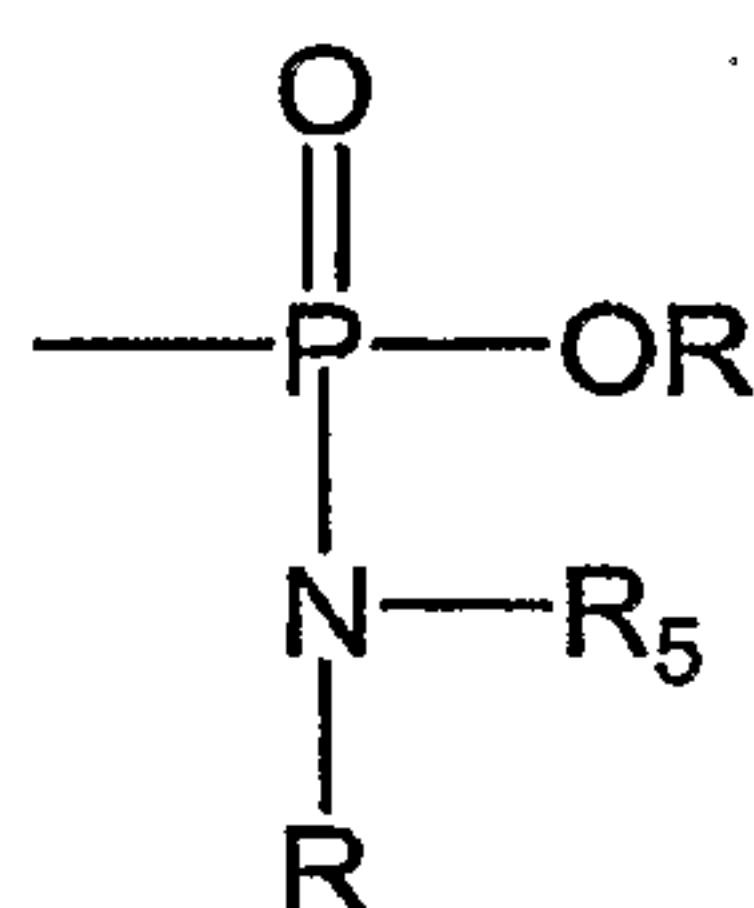
phosphoramidate
