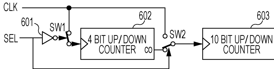
FIG. 3A COUNTER CIRCUIT
