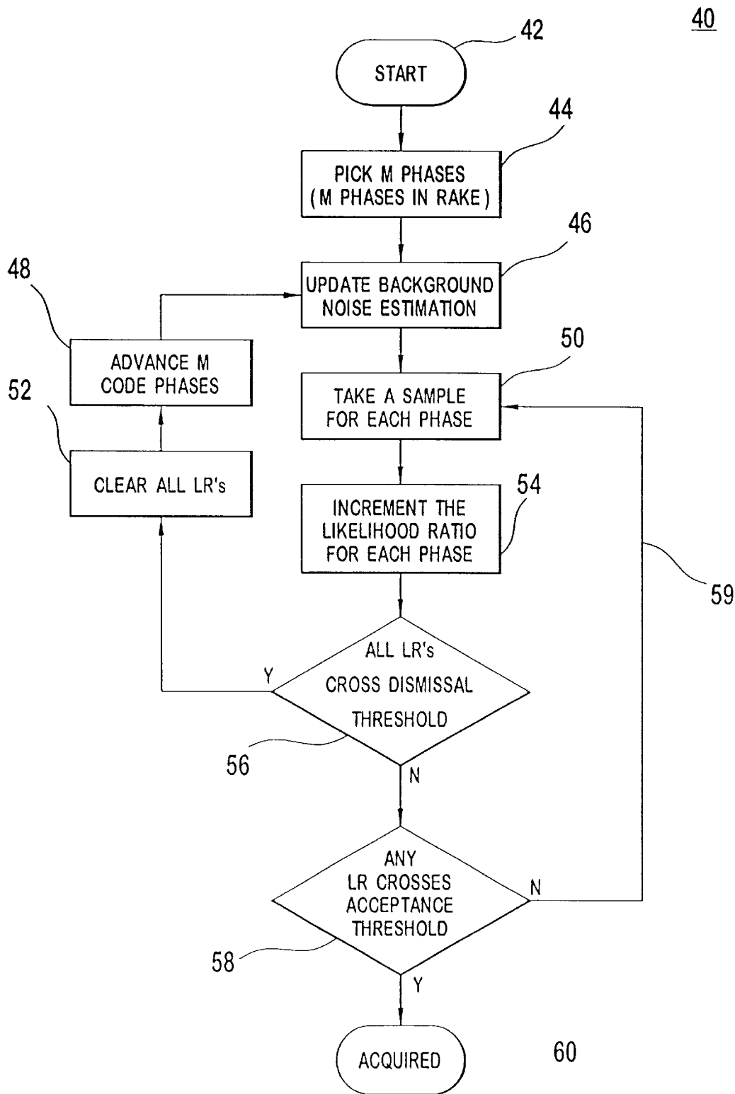
FIG. 2 (PRIOR ART)
