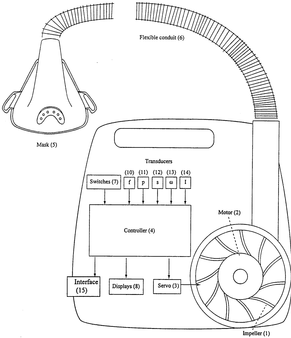
Figure 2: CPAP apparatus
