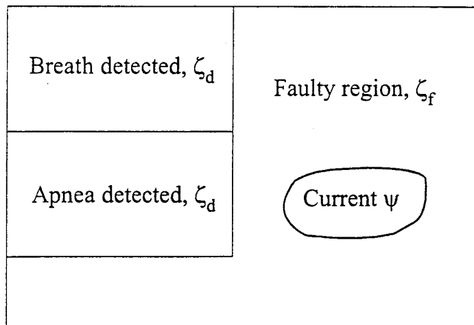
Figure 16: Software fault
