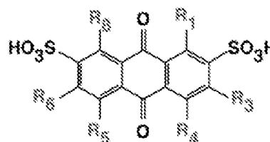
Scheme 1. AQDS screened by theoretical calculations.
