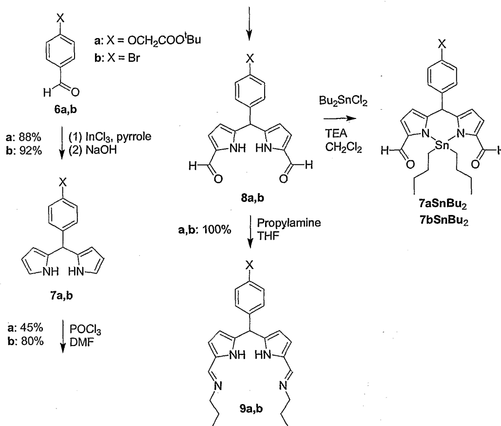
Scheme 2
