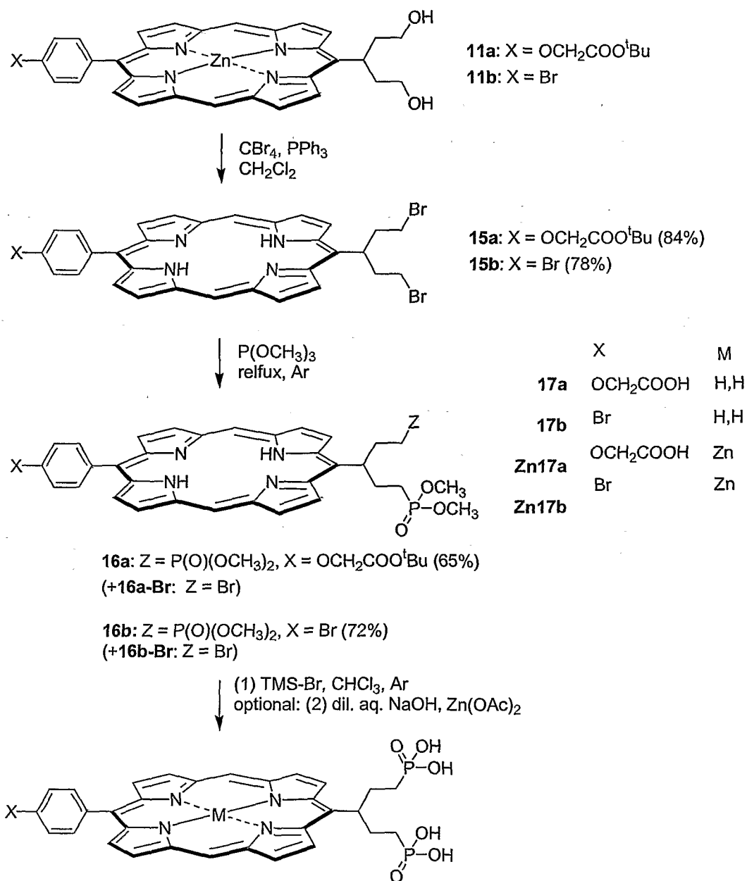
Scheme 6
