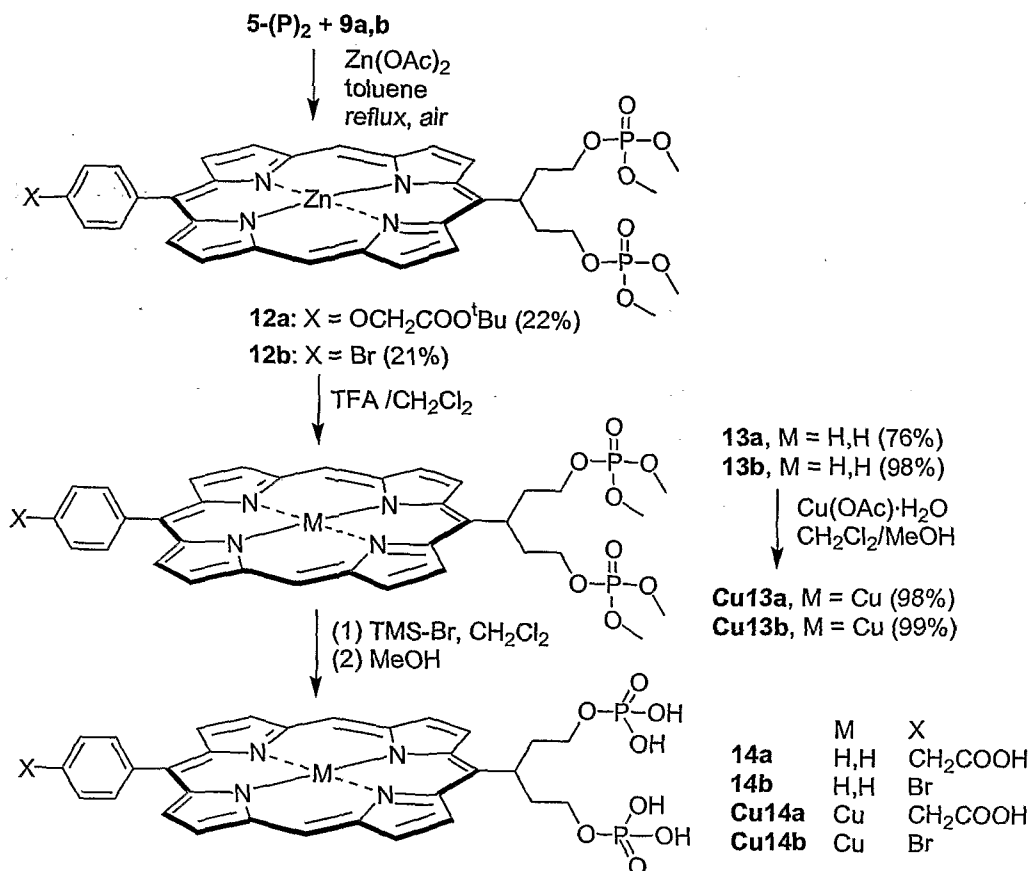
Scheme 5
