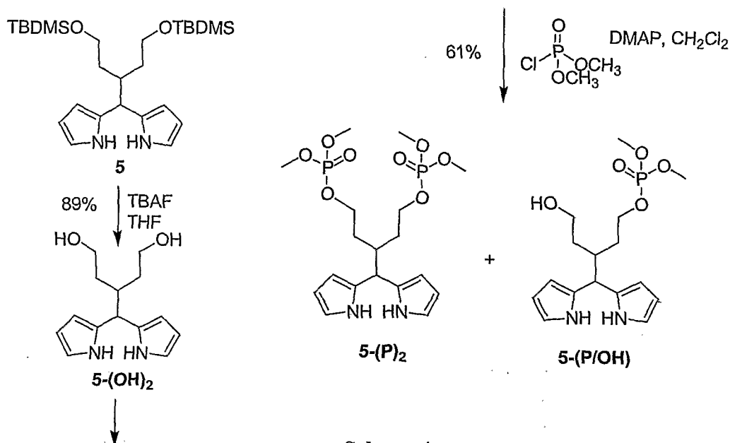
Scheme 4
