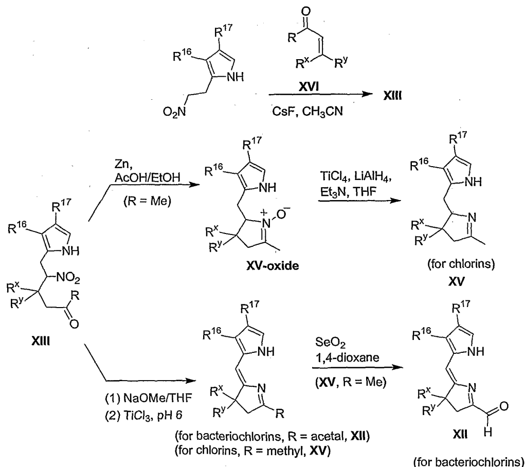
Synthetic Scheme
