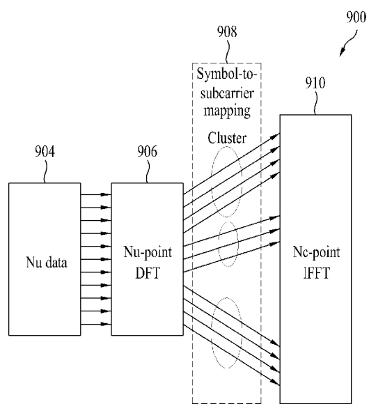
Clusters DFT-s-OFDMA
