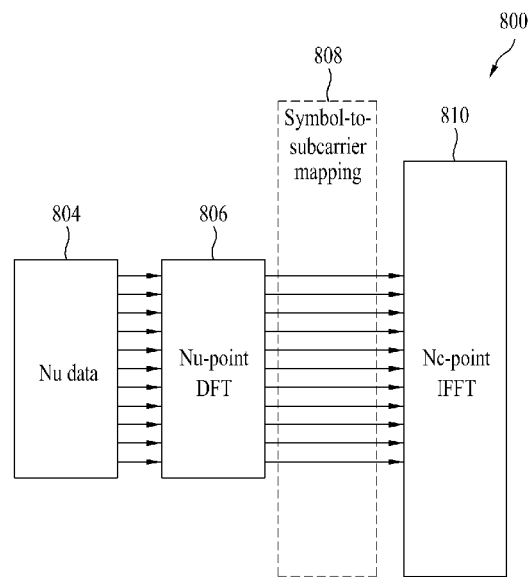
Localized DFT-s-OFDMA
