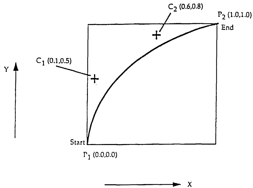
Fig. 10A. Normalized Cubic Bézier Curve
