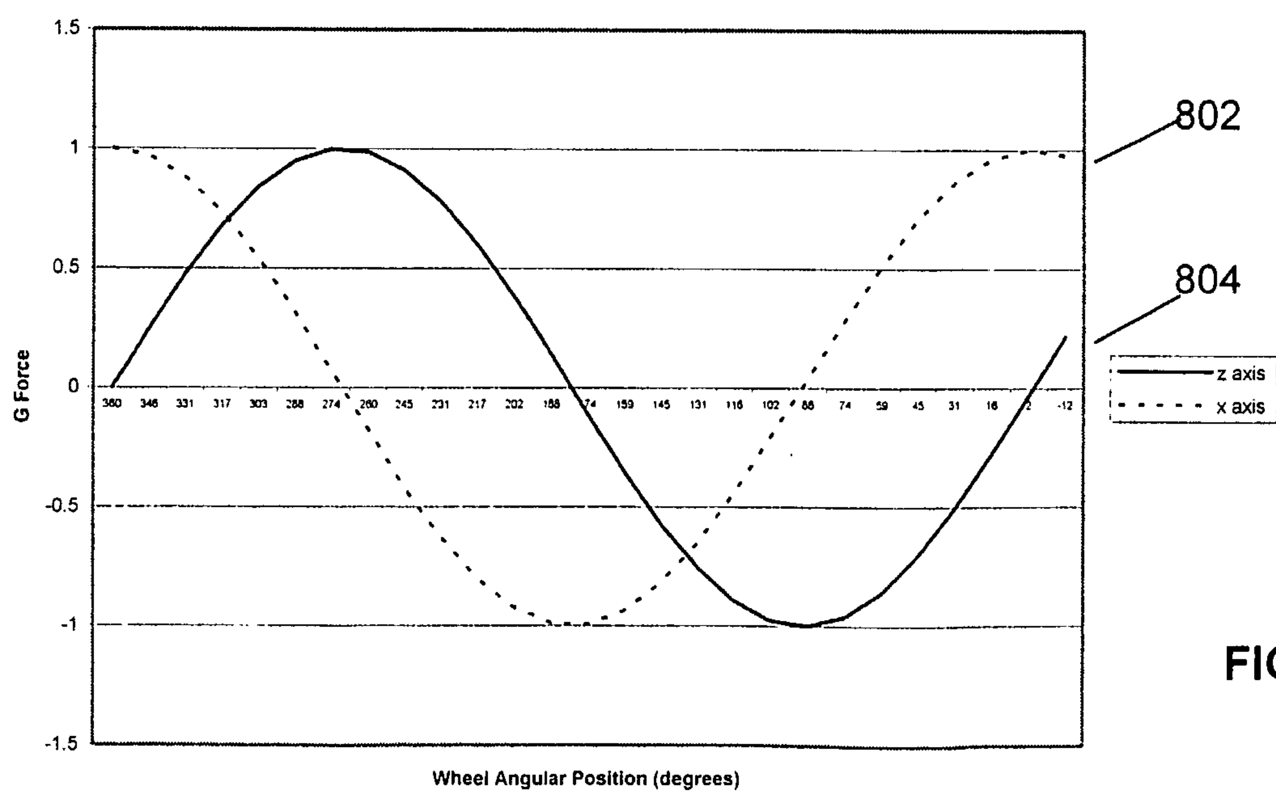
G Force vs Wheel Angular Position (CW)
