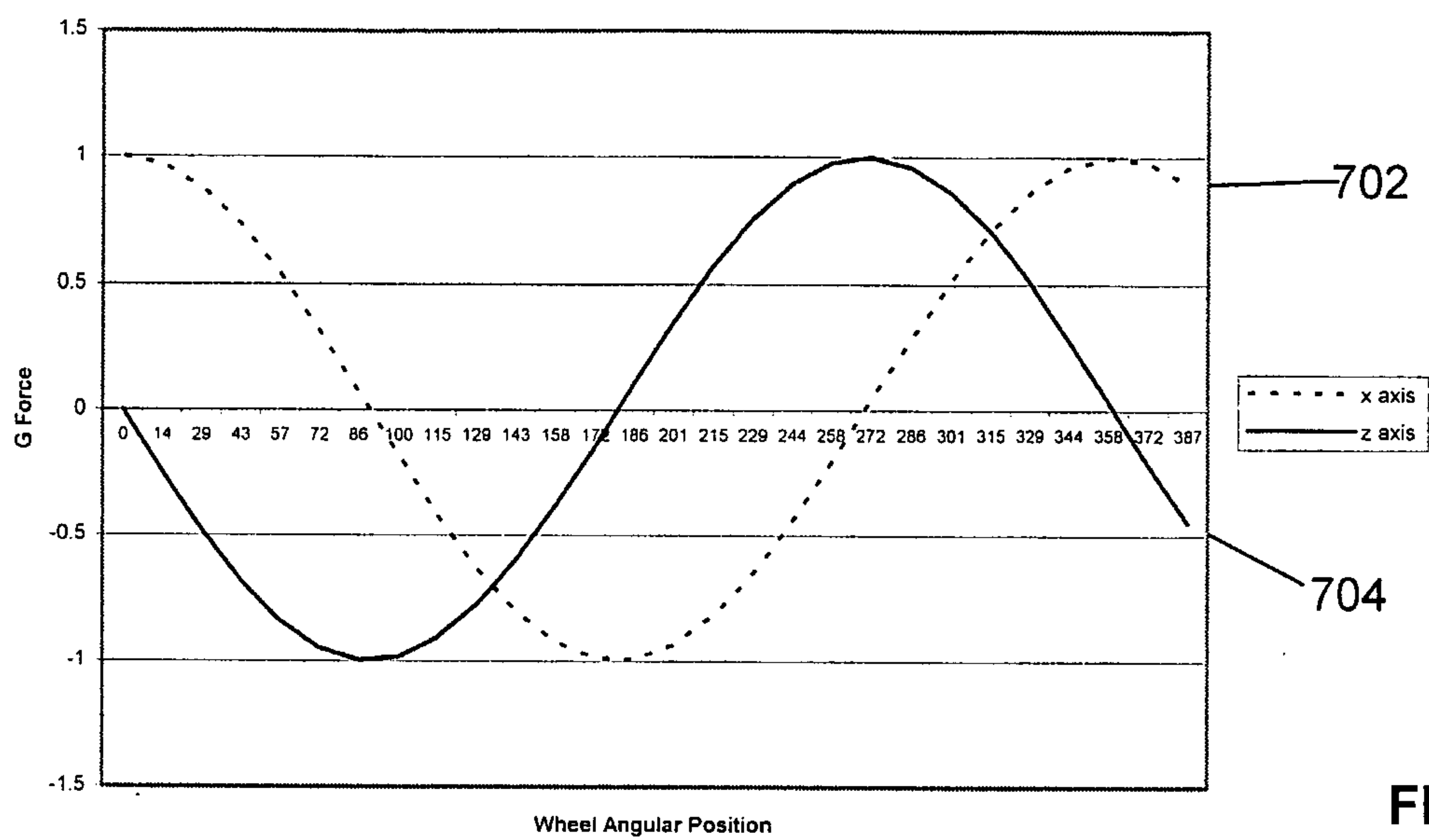
G Force vs Wheel Angular Position (CCW)
