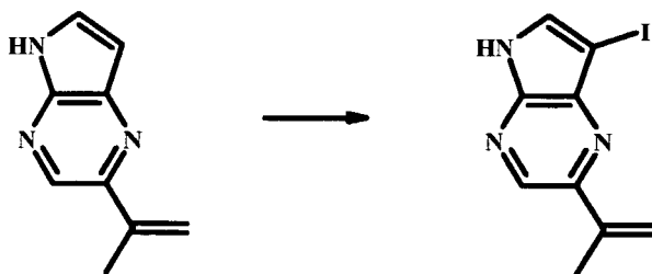
7-Iodo-2-isopropenyl-5H-pyrrolo[2,3-b]pyrazine
