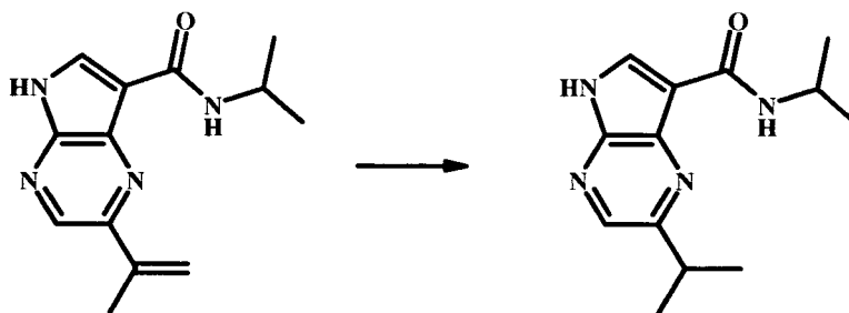
2-Isopropyl-5H-pyrrolo[2,3-b]pyrazine-7-carboxylic acid isopropylamide
