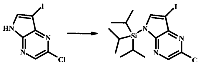
2-Chloro-7-iodo-5-triisopropylsilyl-5H-pyrrolo[2,3-b]pyrazine
