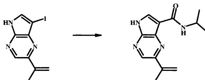
2-Isopropenyl-5H-pyrrolo[2,3-b]pyrazine-7-carboxylic acid isopropylamide
