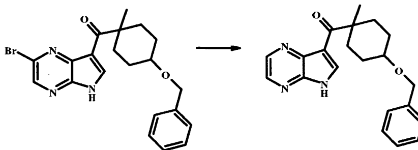
(4-Benzyloxy-1-methyl-cyclohexyl)-(5H-pyrrolo[2,3-b]pyrazin-7-yl)-methanone
