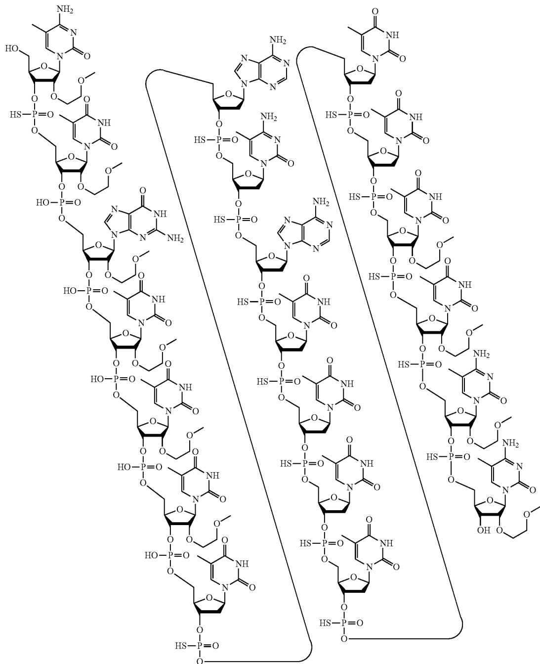
Structure 3. Compound No. 1489494
