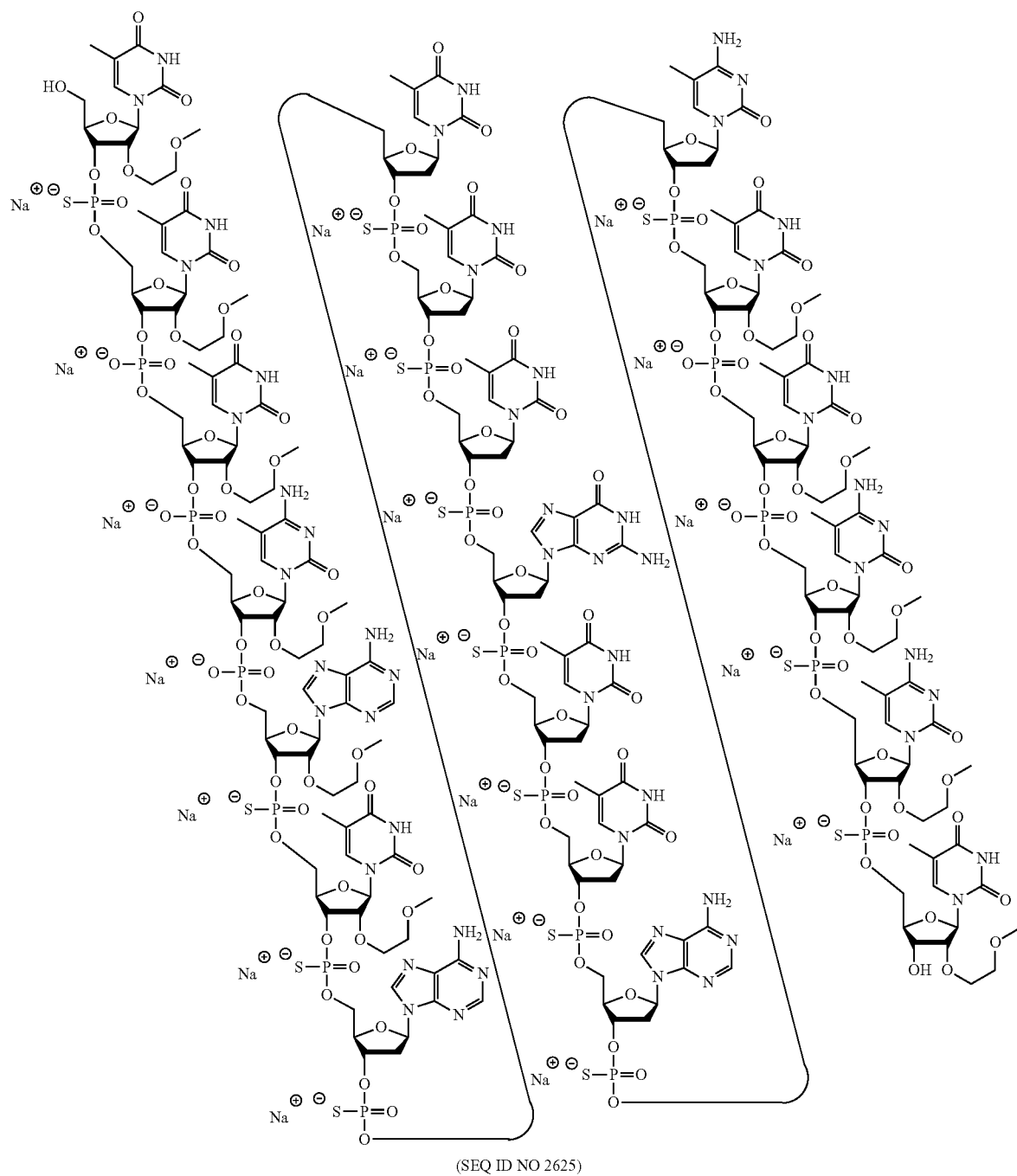
Structure 10. The sodium salt of Compound No. 1492082
