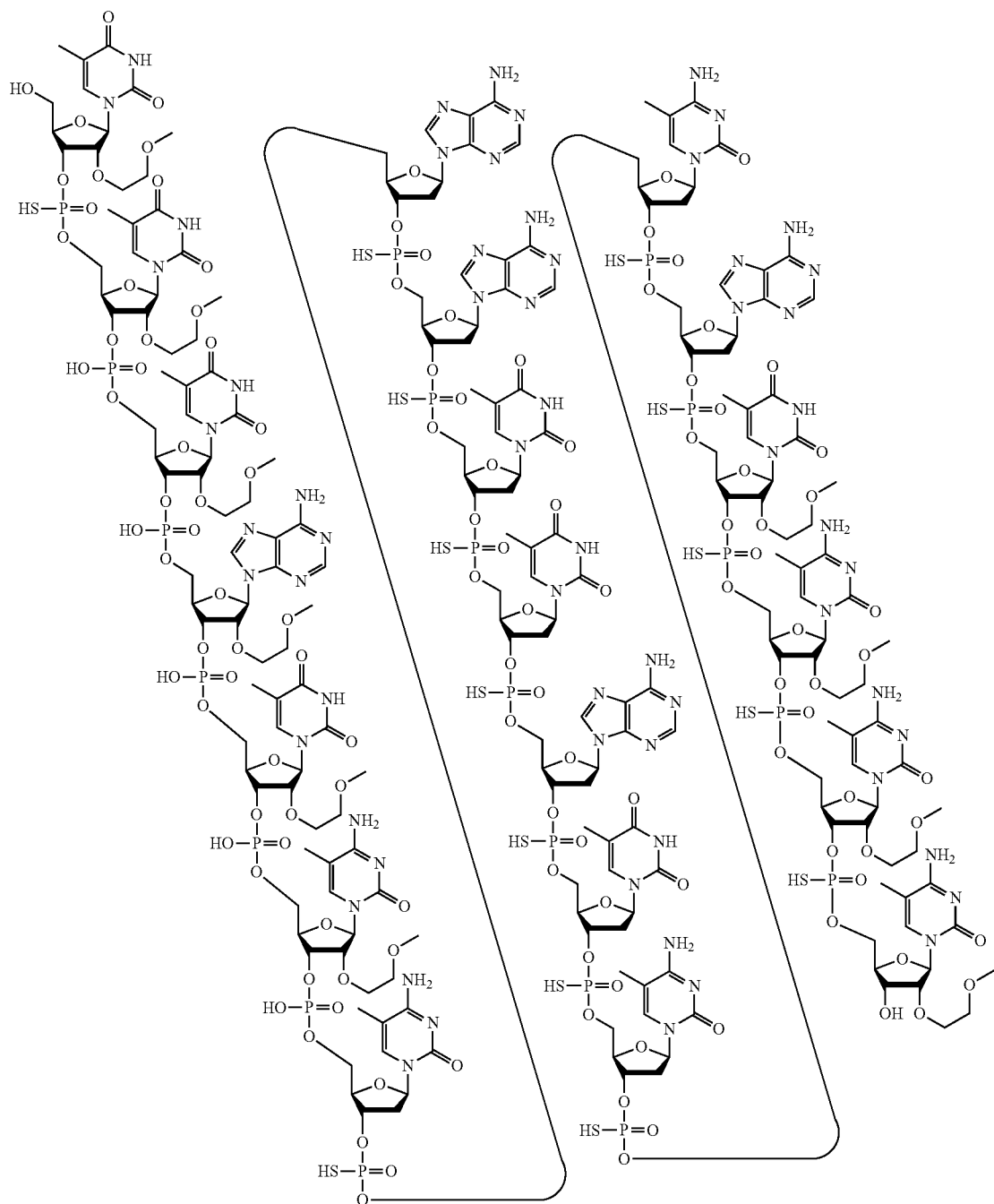
Structure 3. Compound No. 1489552
