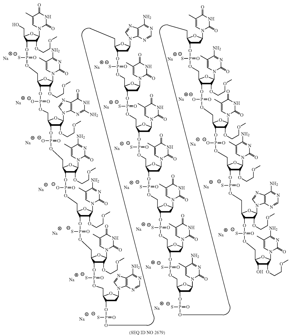
Structure 8. The Sodium salt of Compound No. 1492069
