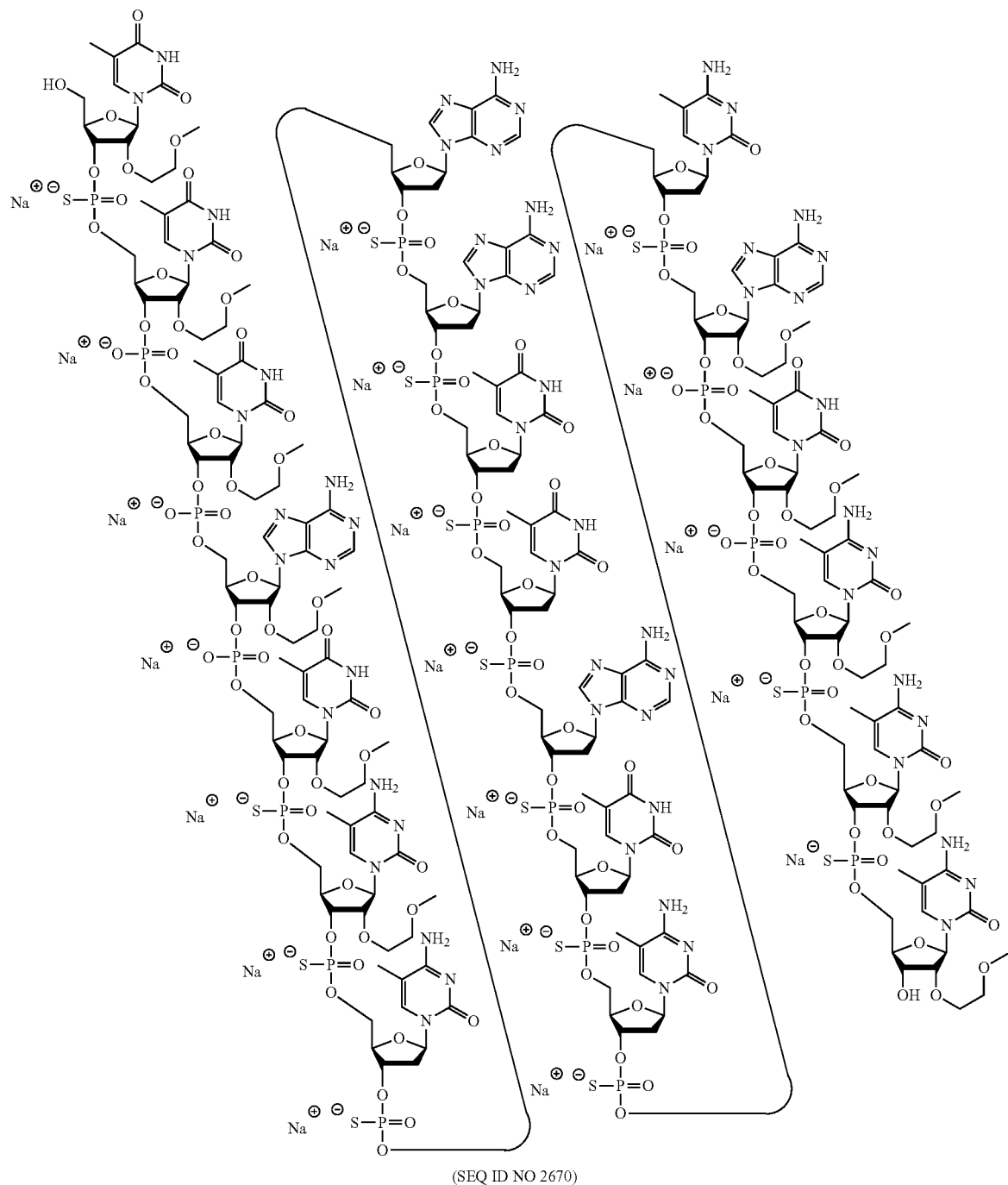
Structure 6. The sodium salt of Compound No. 1489525
