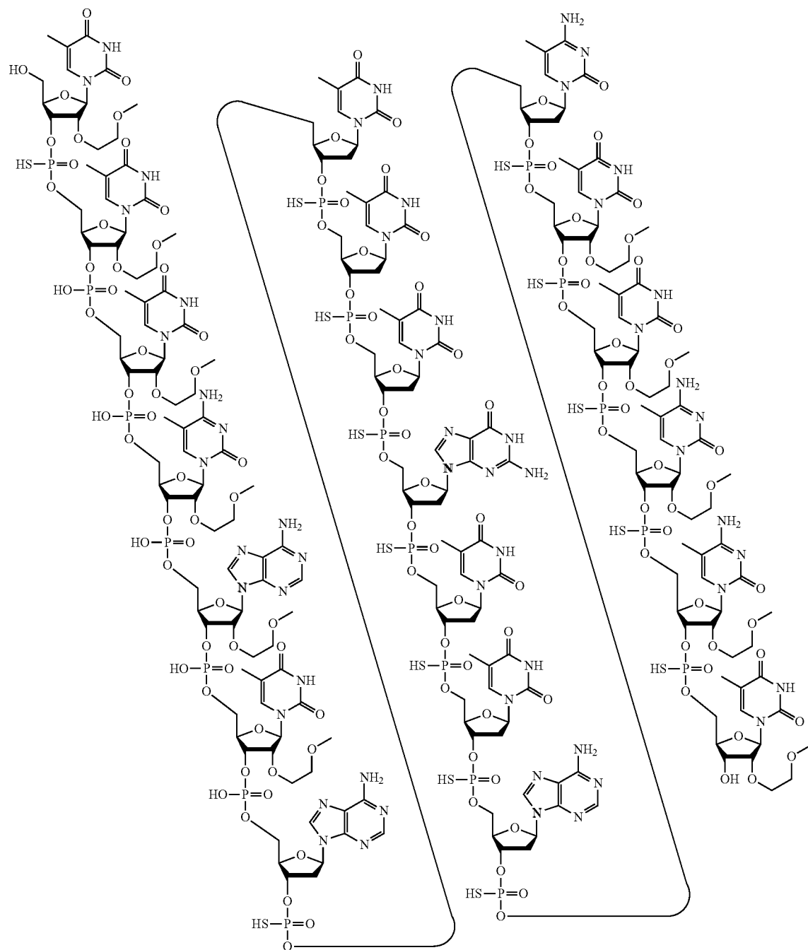
Structure 9. Compound No. 1492082
