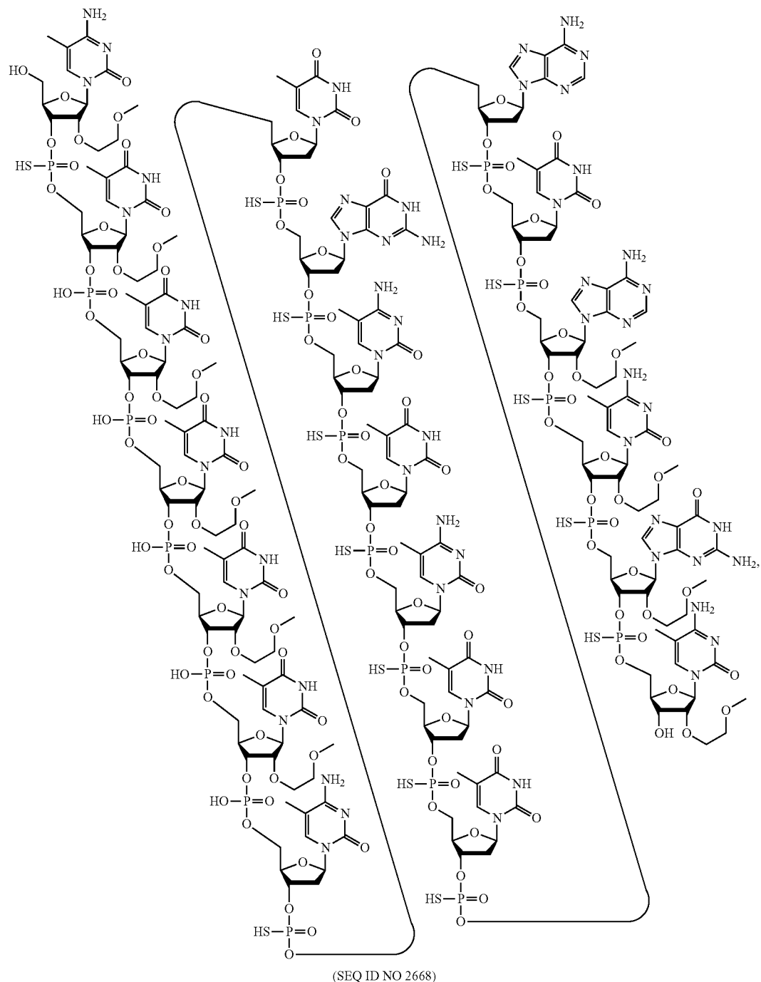
Structure 1. Compound No. 1489477
