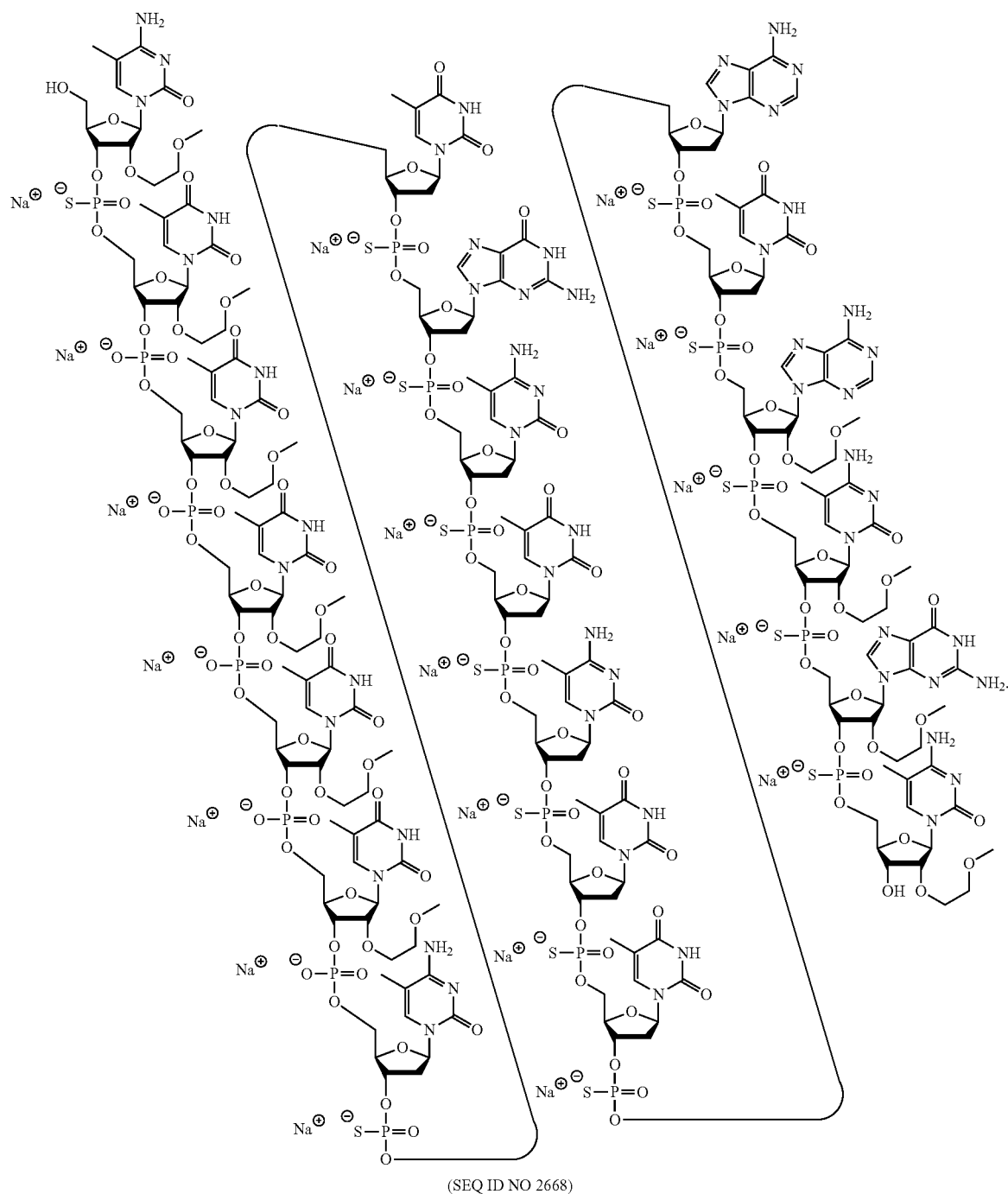
Structure 2. The sodium of Compound No. 1489477
