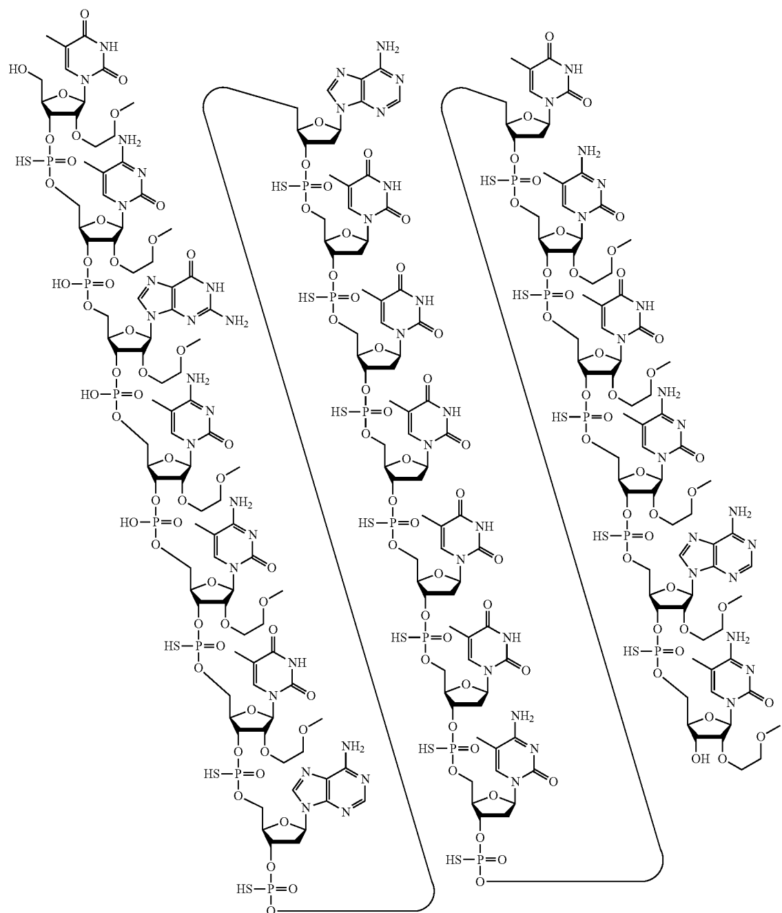
Structure 7. Compound No. 1492069
