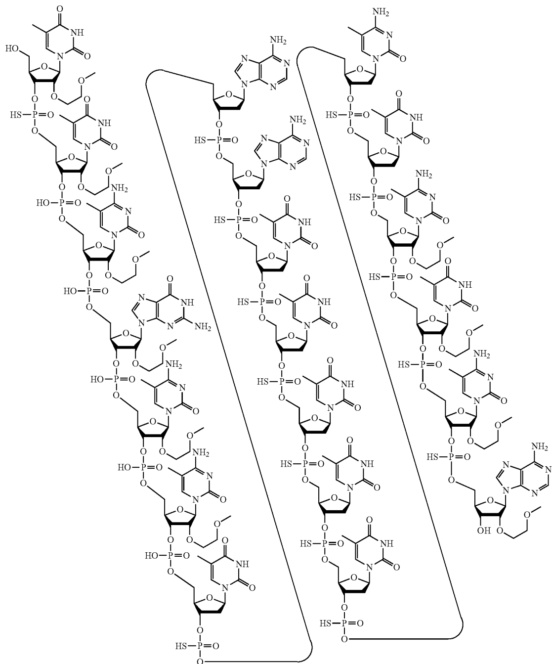
Structure 11. Compound No. 1492131
