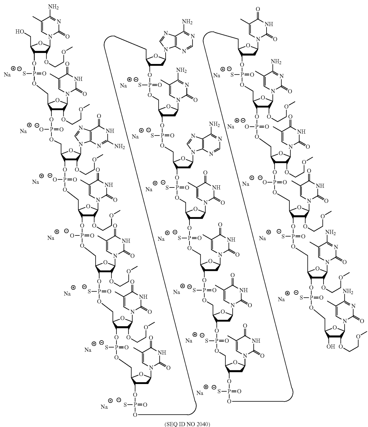
Structure 4. The Sodium salt of Compound No. 1489494
