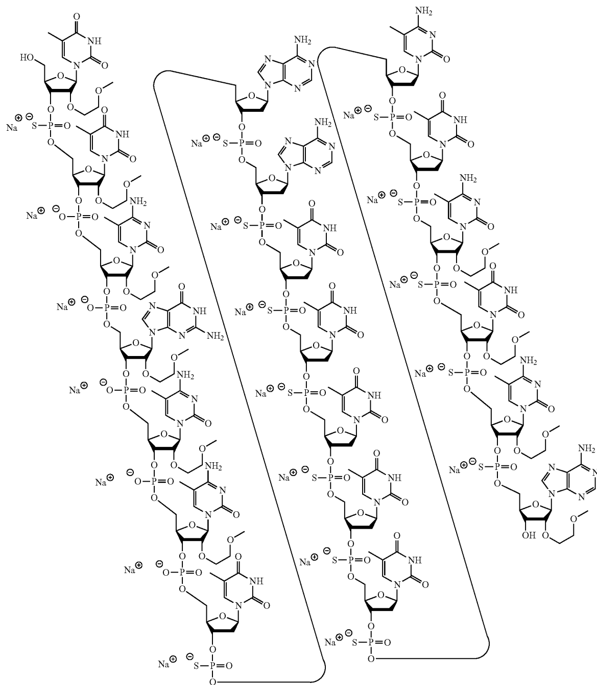
Structure 12. The sodium salt of Compound No. 1492131
