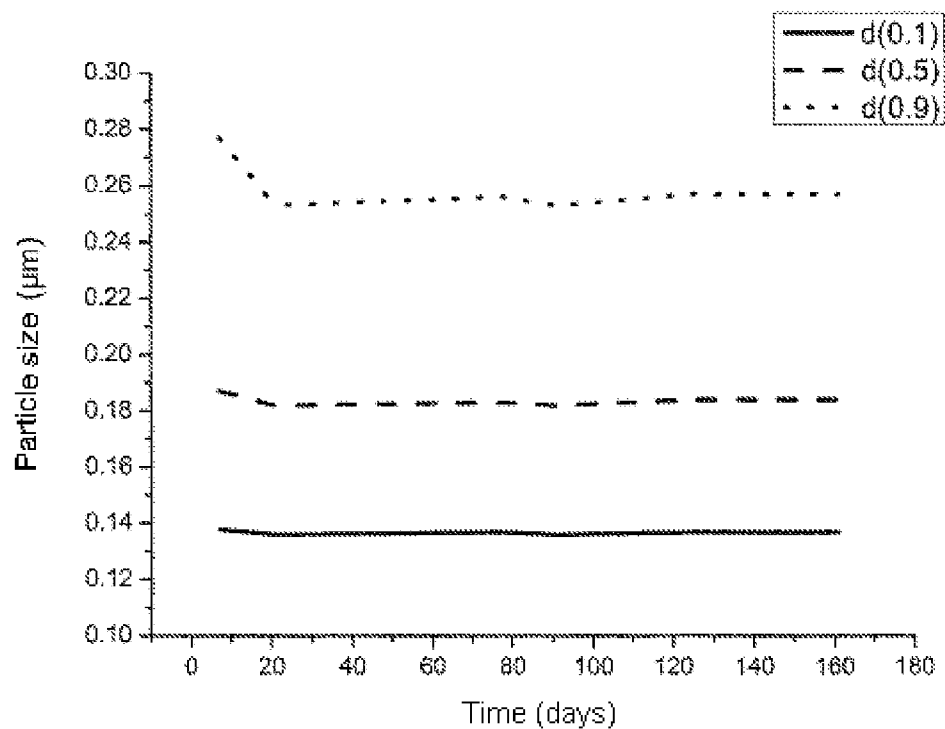
Figure 5. Evolution of the particle size distribution parameters d(0.1) , d(0.5) and d(0.9) against time for a calcium sulphate dihydrate suspension produced in accordance with the invention from Example 1.
