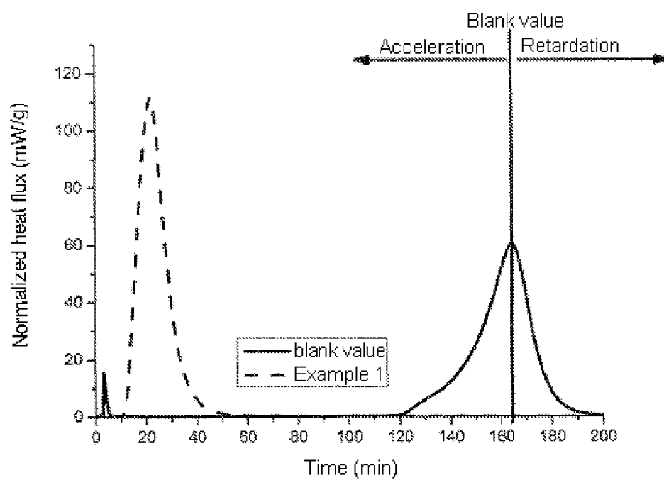
Figure 1. Typical heat flux curves of the retarded blank system without accelerator (solid line) and of the accelerated system (Example 1, broken line).
