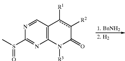
Scheme 4
