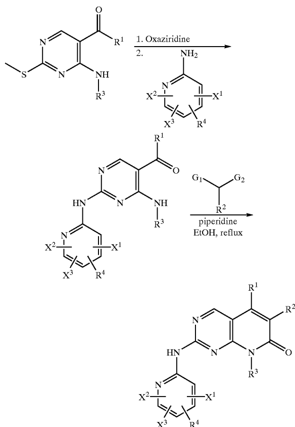
Scheme 13
