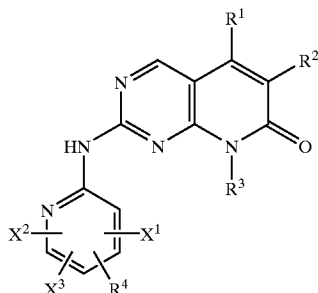
Scheme 13
