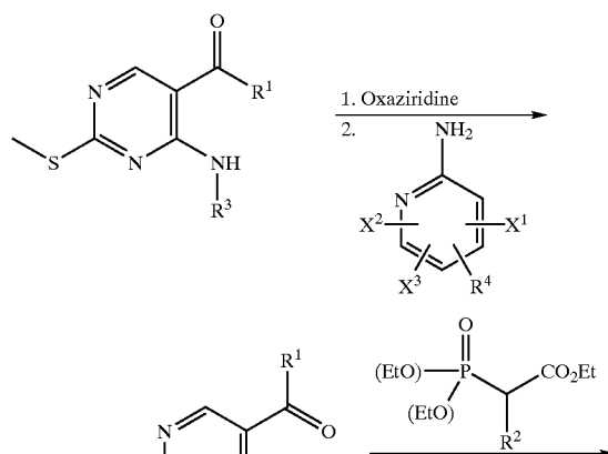
Scheme 11
