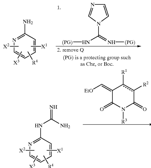
Scheme 5
