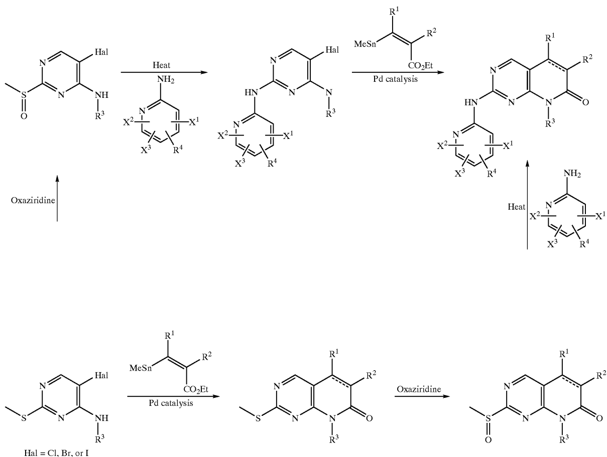
Scheme 6
