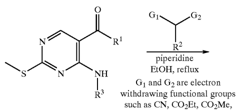
Scheme 10
