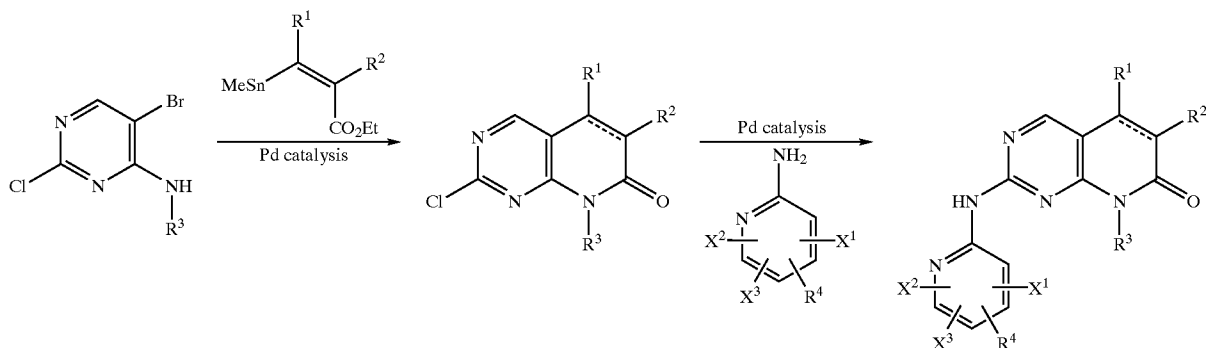
-continued Scheme 7
