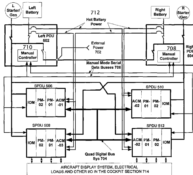
Twin Generator, 4 SPDU Configuration 700
