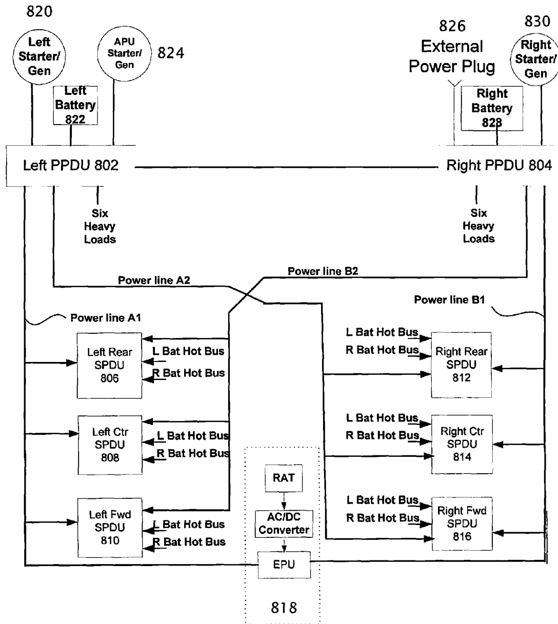
High Availability Two Generator System 800
