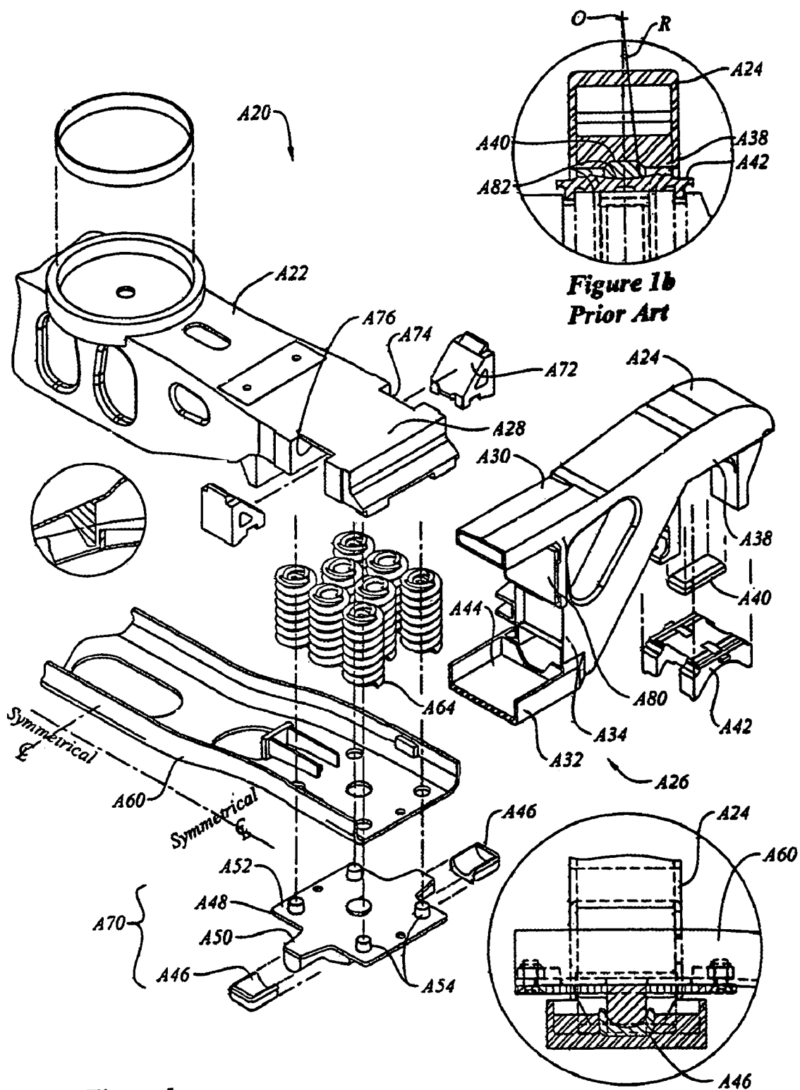
Figure 1c Prior Art
