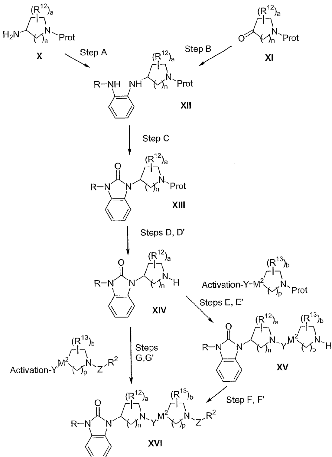
SCHEME 1. General Method for Preparation of Compounds of Formula XVI
