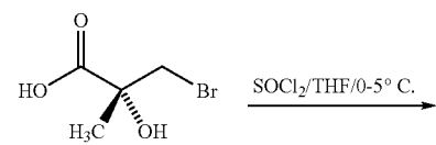
(R)-3-bromo-2-hydroxy-2-methylpropanoic acid
