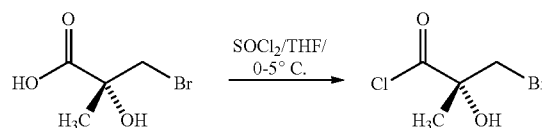
(R)-3-bromo-2-hydroxy-2-methylpropanoic acid R-18
