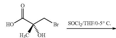
(R)-3-bromo-2-hydroxy-2-methylpropanoic acid
