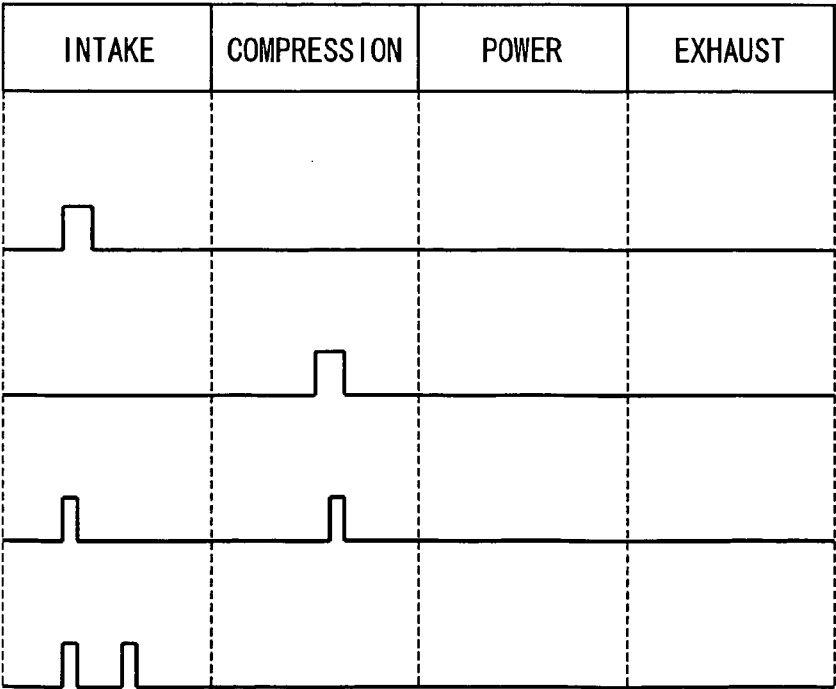
FIG. 15A INJECTION PULSE
