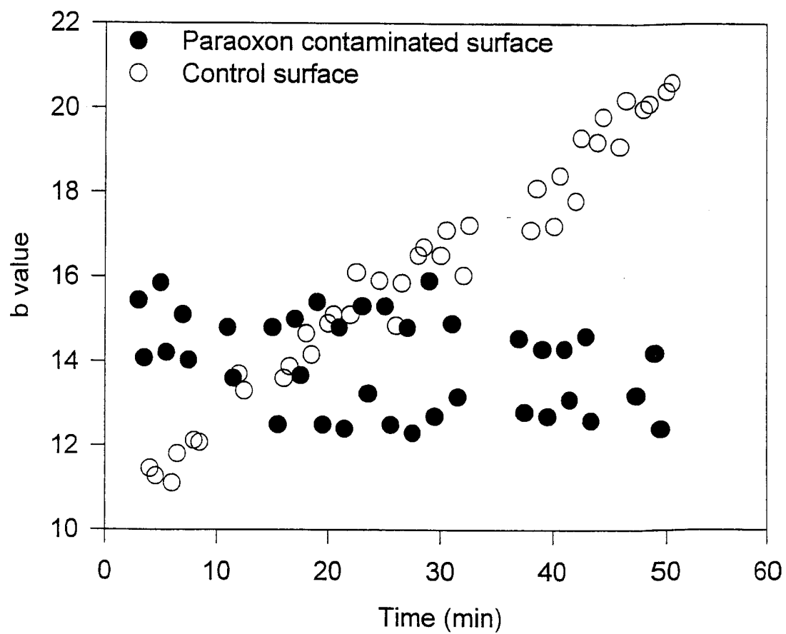
Figure 4. Detection of paraoxon at a surface using BChE-containing polymers.
