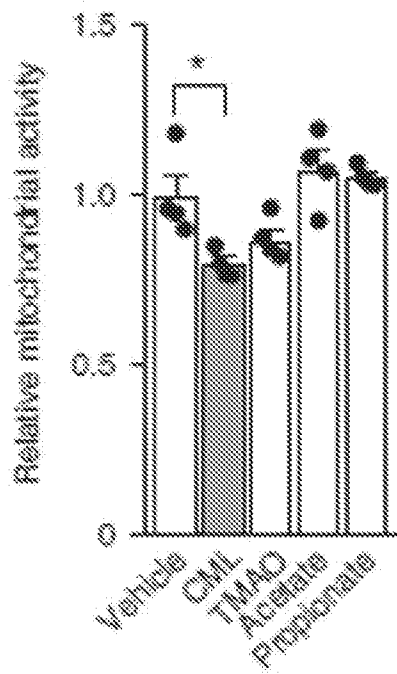
Mitochondrial Activity
