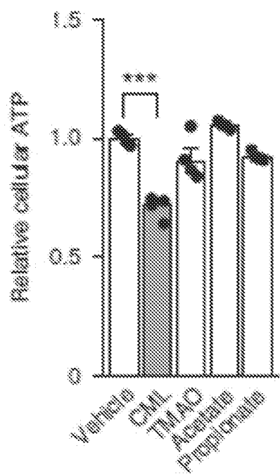
ATP levels
