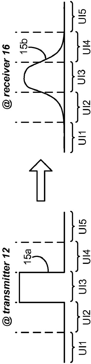
Figure 2 (Prior Art)
