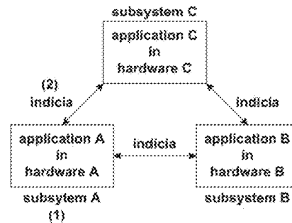
Figure 15b: Heterogeneous Indicia Engine (HIE) TMR Configuration
