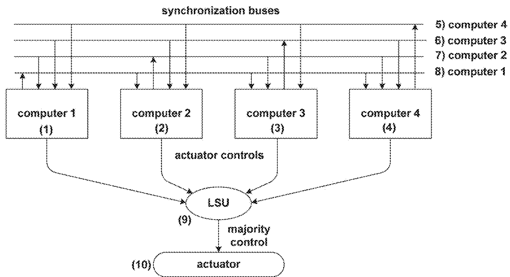
Figure 14: Prior-Art - NASA Space Shuttle
