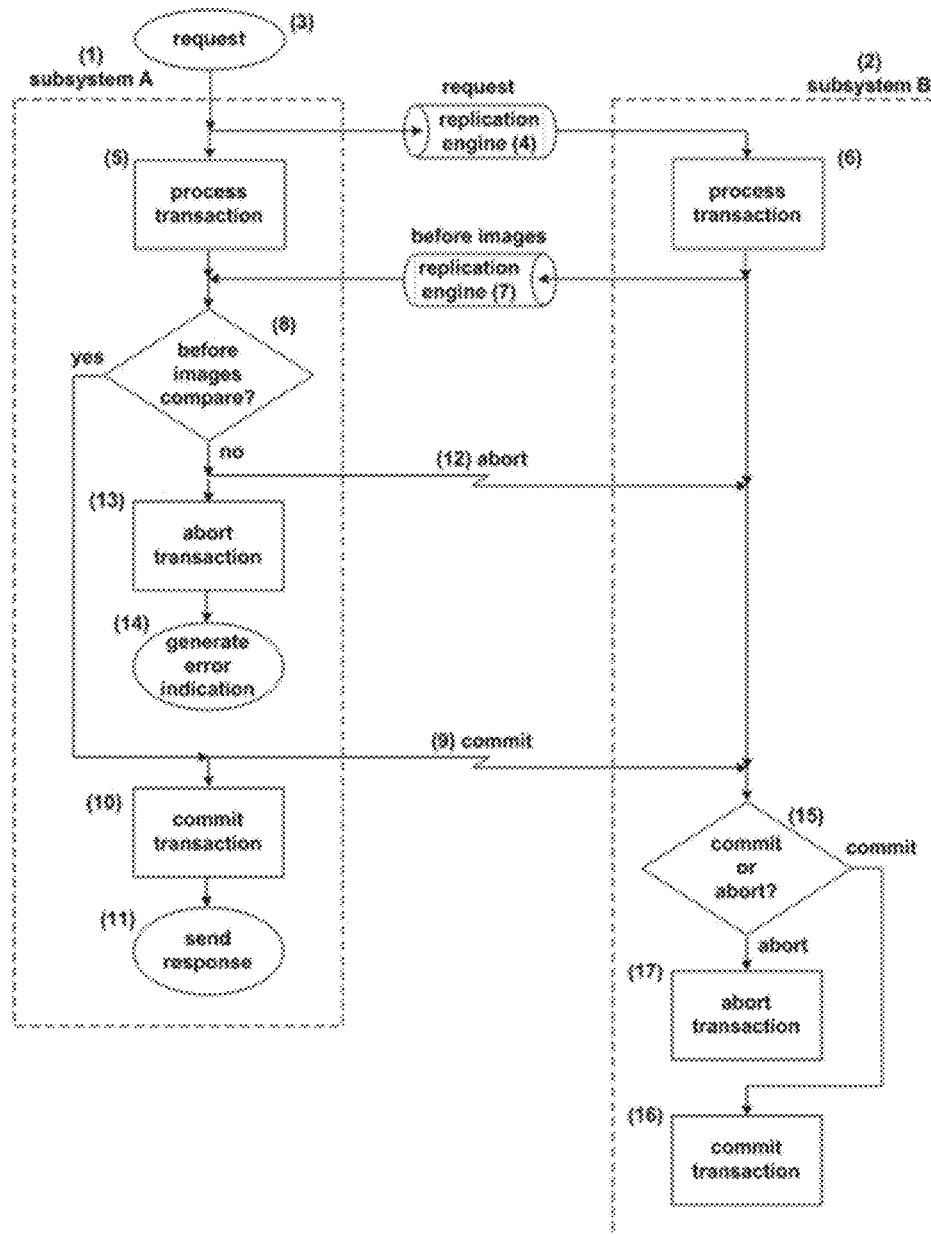
Figure 21: Alternative Embodiment for HIE
