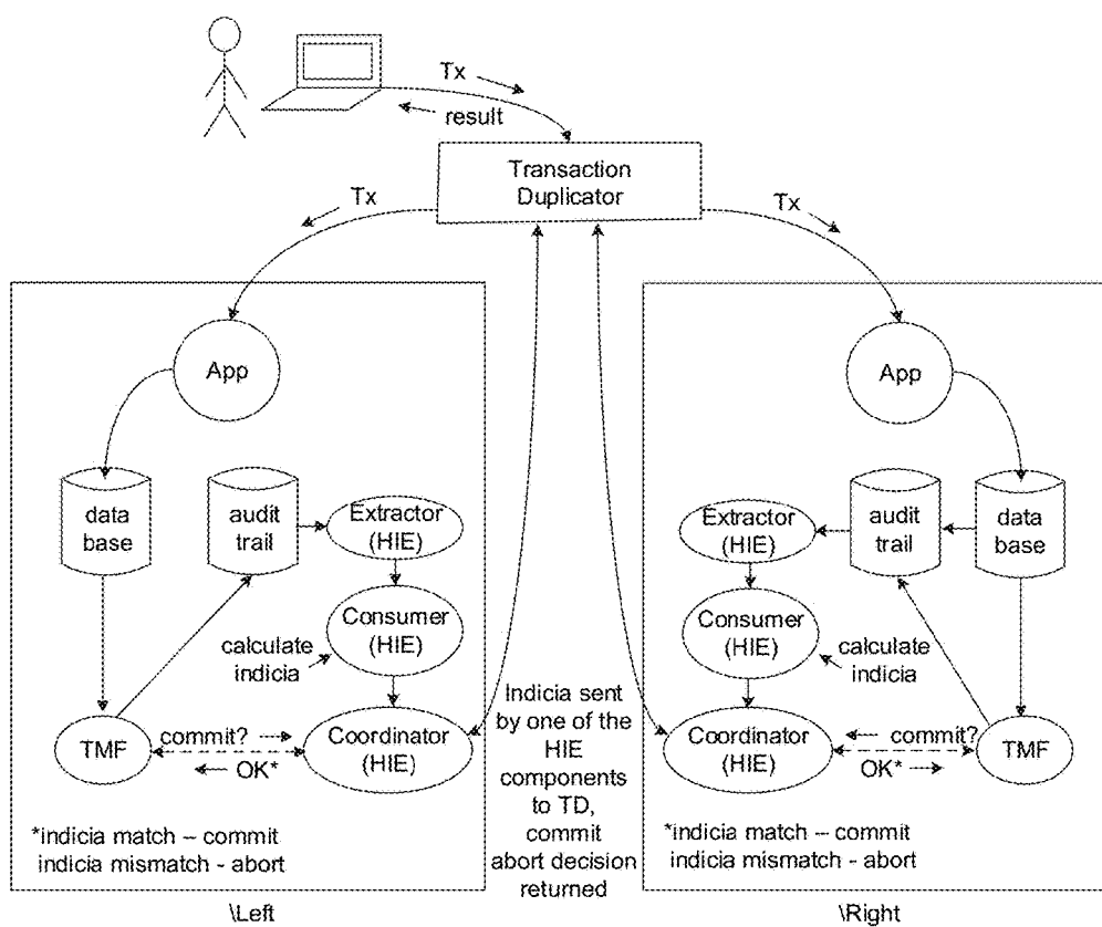
Figure 28: Internal structure of the HIE with TD accomplishing the indicia matching
