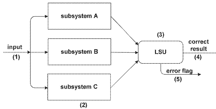
Figure 10: Prior Art - Logical Synchronization Unit (LSU)
