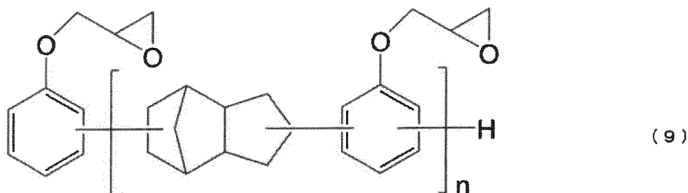
[Chem 35]
