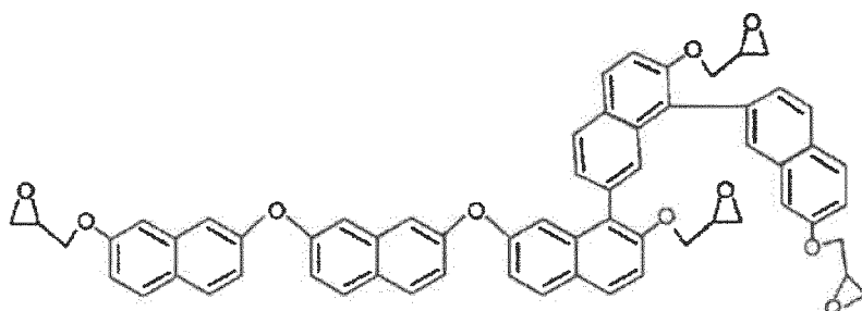
[Chem 27]
