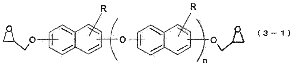
[Chem 22]
