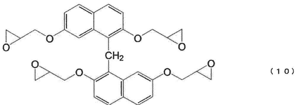
[Chem 36]
