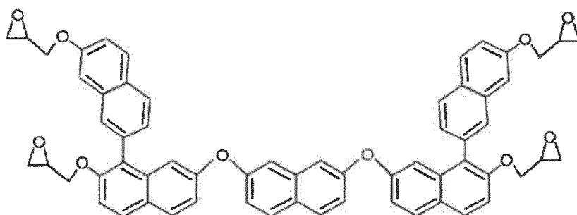
[Chem 27]
