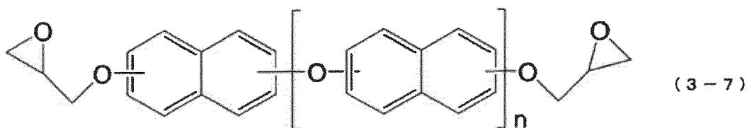
[Chem 34]
