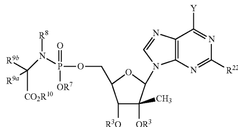
Formula IVa
