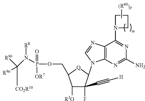
Formula IIIb'
