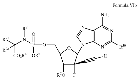
Formula VIb
