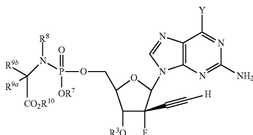
Formula IIIb
