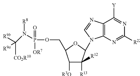
Formula III
