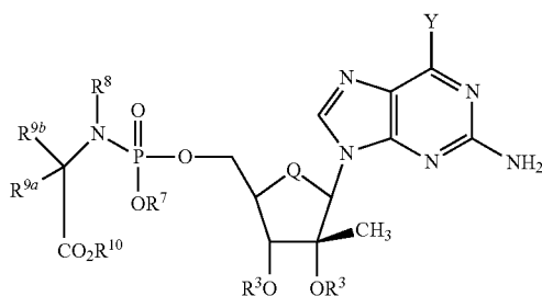
Formula IIIa
