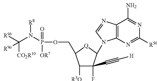
Formula VIb
