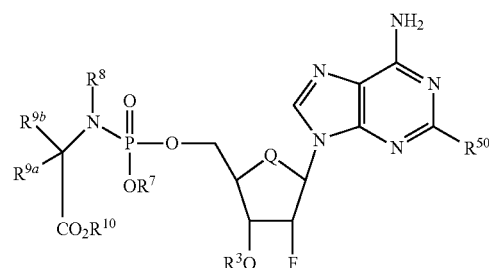
Formula VIc
