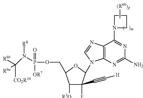
Formula IIIb'
