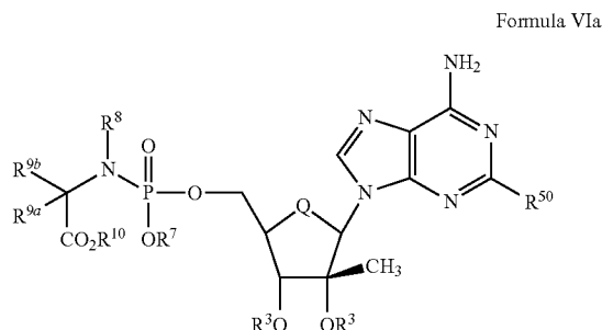
Formula VIa
