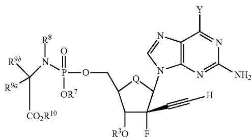
Formula IIIb
