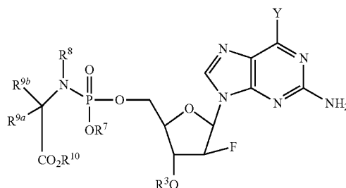
Formula IIId
