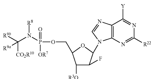
Formula IVd
