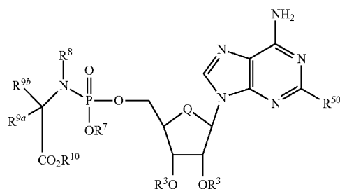
Formula Vie
