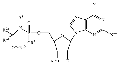
Formula IIIc
