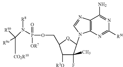
Formula VIf
