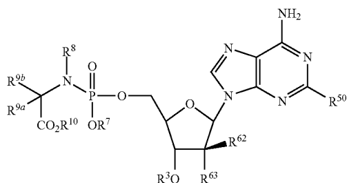
Formula VI
