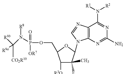
Formula IVe
