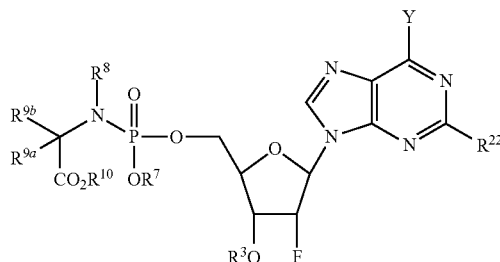
Formula IVc
