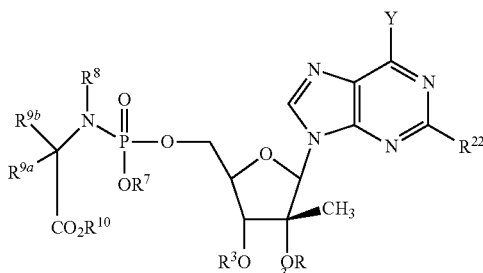
Formula IVa
