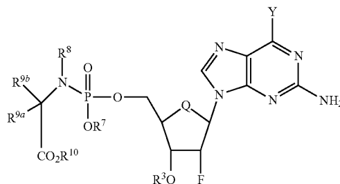
Formula IIIc
