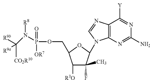
Formula IIIe
