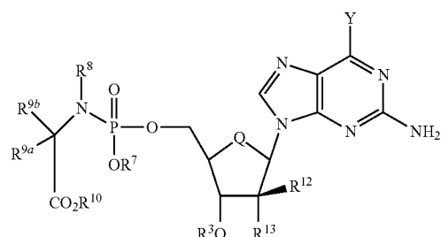
Formula III
