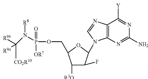
Formula IIIc
