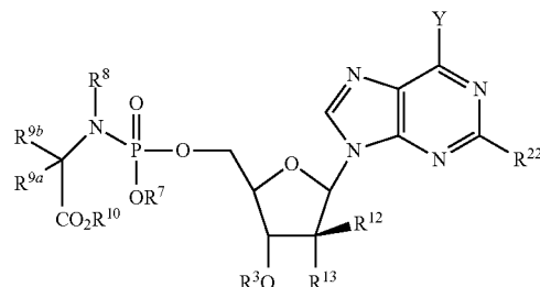
Formula IV
