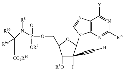
Formula IVb
