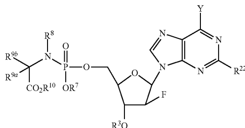
Formula IVd
