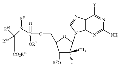
Formula IIIE
