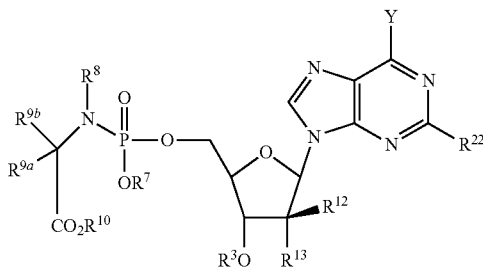
Formula IV
