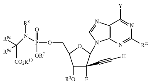
Formula IVb
