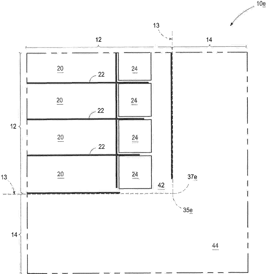
FIG. 8 Predecessor Substrate
