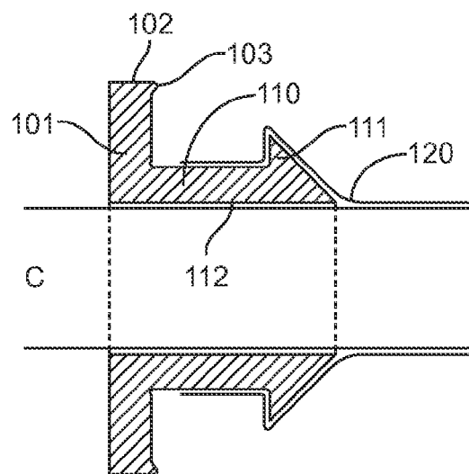
Section A-A (Figure not to scale)
