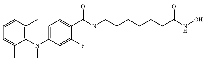
4-((2,6-dimethylphenyl)(methyl)amino)-2-fluoro-N-(7-(hydroxyamino)-7-oxoheptyl)-N-methylbenzamide IC_{50}(nM) HDAC6 = 9 HDAC3 = 148
