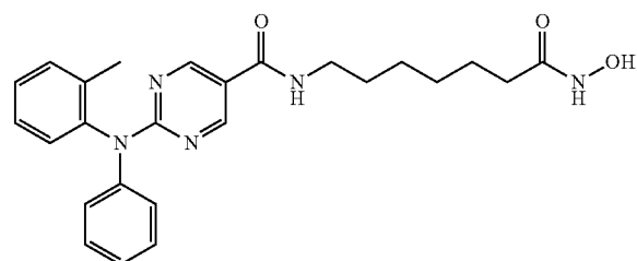
N-(7-(hydroxyamino)-7-oxoheptyl)-2-(phenyl(o-tolyl)amino)pyrimidine-5-carboxamide
