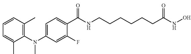
4-((2,6-dimethylphenyl)(methyl)amino)-2-fluoro-N-(7-(hydroxyamino)-7-oxoheptyl)benzamide IC_{50}(nM) HDAC6 = 5 HDAC3 = 107
