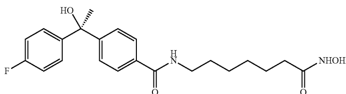
4-(1-(4-fluorophenyl)-1-hydroxyethyl)-N-(7-(hydroxyamino)-7-oxoheptyl)benzamide IC_{50}(nM) HDAC6 = 3 HDAC3 = 37
