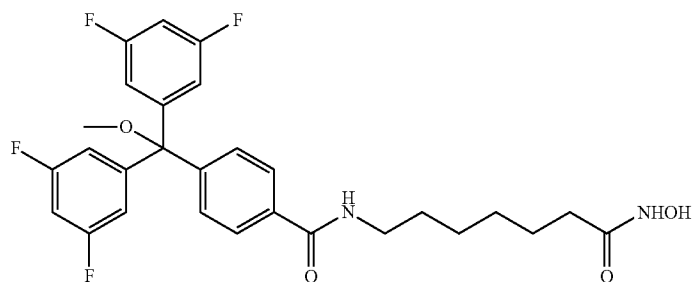
4-(bis(3,5-difluorophenyl)(hydroxy)methyl)-N-(7-(hydroxyamino)-7-oxoheptyl)benzamide IC_{50}(nM) HDAC6 = 20 HDAC3 = 679
