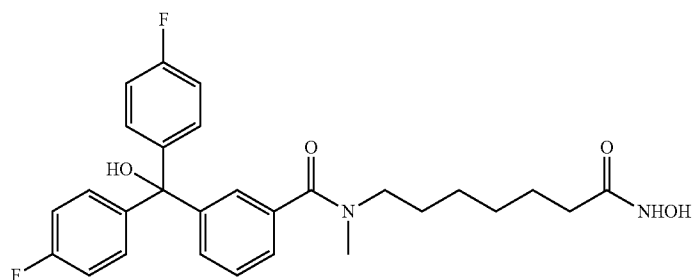
3-(bis(4-fluorophenyl)(hydroxy)methyl)-N-(7-(hydroxyamino)-7-oxoheptyl)-N-methylbenzamide IC_{50} (nM) HDAC6 = 72 HDAC3 = 349
