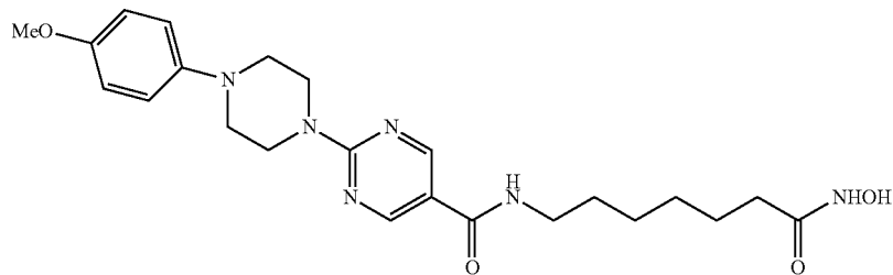
N-(7-(hydroxyamino)-7-oxoheptyl)-2-(4-(4-methoxyphenyl)piperazin-1-yl)pyrimidine-5-carboxamide IC_{50} (nM) HDAC6 = 4 HDAC3 = 58
