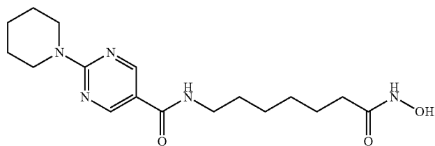
N-(7-(hydroxyamino)-7-oxoheptyl)-2- (piperidin-1-yl)pyrimidine-5-carboxamide IC 50 (nM) HDAC6 = 5 HDAC3 = 23
