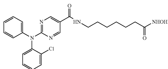
2-((2-chlorophenyl)(phenyl)amino)-N-(7-(hydroxyamino)-7-oxoheptyl)pyrimidine-5-carboxamide
