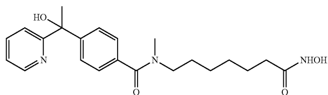
4-(1-(1-hydroxy-1-(pyridin-2-yl)ethyl)-N-(7-(hydroxyamino)-7-oxoheptyl)-N-methylbenzamide IC_{50}(nM) HDAC6 = 36 HDAC3 = 501
