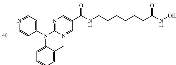
N-(7-(hydroxyamino)-7-oxoheptyl)-2-(pyridin-4-yl(o-tolyl)amino)pyrimidine-5-carboxamide
