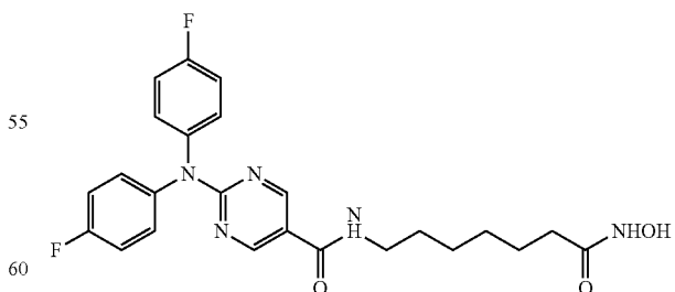
2-(bis(4-fluorophenyl)amino)-N-(7-(hydroxyamino)-7-oxoheptyl)pyrimidine-5-carboxamide
