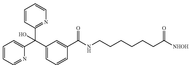
N-(7-(hydroxyamino)-7-oxoheptyl)-3-(hydroxydipyridin-2-ylmethyl)benzamide IC_{50}(nM) HDAC6 = 41 HDAC3 = 285
