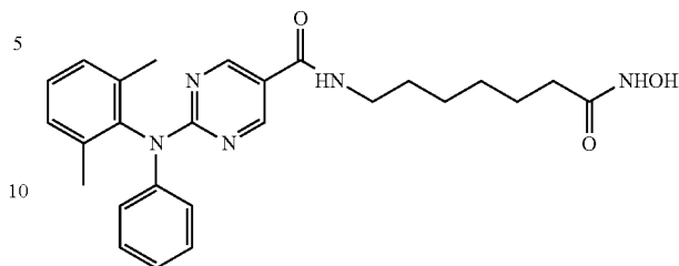
2-((2,6-dimethylphenyl)(phenyl)amino)-N-(7-(hydroxyamino)-7-oxoheptyl)pyrimidine-5-carboxamide
