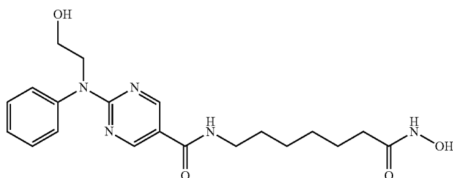
N-(7-(hydroxyamino)-7-oxoheptyl)-2-(2-(2-hydroxyethyl)phenylamino)pyrimidine-5-carboxamide IC_{50}(nM) HDAC6 = 8 HDAC3 = 75
