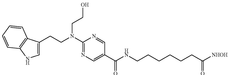
2-((2-(1H-indol-3-yl)ethyl)(2-hydroxyethyl)amino)-N-(7-(hydroxyamino)-7-oxoheptyl)pyrimidine-5-carboxamide IC_{50} (nM) HDAC6 = 3 HDAC3 = 35
