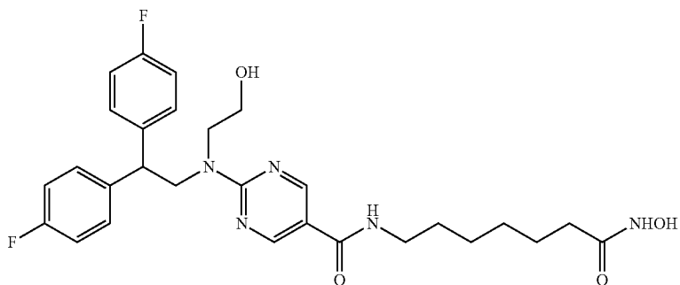
2-((2,2-bis(4-fluorophenyl)ethyl)(2-hydroxyethyl)amino)-N-(7-(hydroxyamino)-7-oxoheptyl)pyrimidine-5-carboxamide IC_{50} (nM) HDAC6 = 8 HDAC3 = 64
