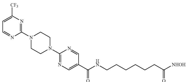
N-(7-(hydroxyamino)-7-oxoheptyl)-2-(4-(trifluoromethyl)pyrimidin-2-yl)piperazin-1-yl)pyrimidine-5-carboxamide IC_{50} (nM) HDAC6 = 7 HDAC3 = 54
