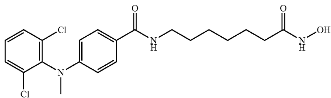
4-((2,6-dichlorophenyl)(methyl)amino)-N-(7-(hydroxyamino)-7-oxoheptyl)benzamide IC_{50}(nM) HDAC6 = 3 HDAC3 = 29
