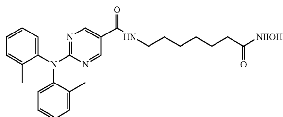
2-(di-o-tolylamino)-N-(7-(hydroxyamino)-7-oxoheptyl)pyrimidine-5-carboxamide
