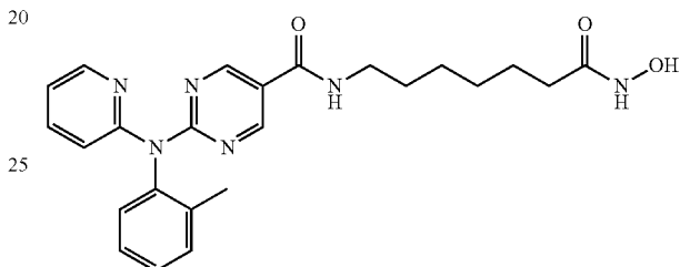
N-(7-(hydroxyamino)-7-oxoheptyl)-2-(pyridin-2-yl(o-tolyl)amino)pyrimidine-5-carboxamide
