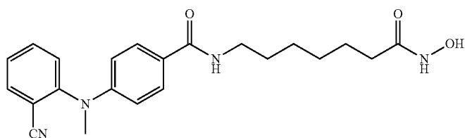
4-(2-cyanophenyl)(methyl)amino)-N-(7-(hydroxyamino)-7-oxoheptyl)benzamide IC_{50} (nM) HDAC6 = 4 HDAC3 = 23
