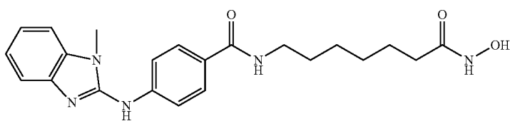
N-(7-(hydroxyamino)-7-oxoheptyl)-4-(1-methyl-1H-benzo[d]imidazol-2-ylamino)benzamide IC_{50} (nM) HDAC6 = 9 HDAC3 = 57
