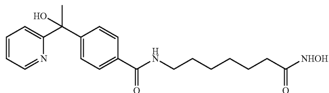
4-(1-(1-hydroxy-1-(pyridin-2-yl)ethyl)-N-(7-(hydroxyamino)-7-oxoheptyl)benzamide IC_{50}(nM) HDAC6 = 7 HDAC3 = 134
