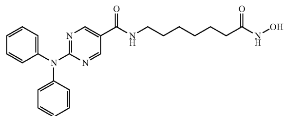
2-(diphenylamino)-N-(7-(hydroxyamino)-7-oxoheptyl)pyrimidine-5-carboxamide
