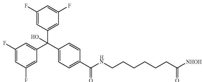
4-(bis(3,5-difluorophenyl)(hydroxy)methyl)-N-(7-(hydroxyamino)-7-oxoheptyl)benzamide IC_{50}(nM) HDAC6 = 4 HDAC3 = 208
