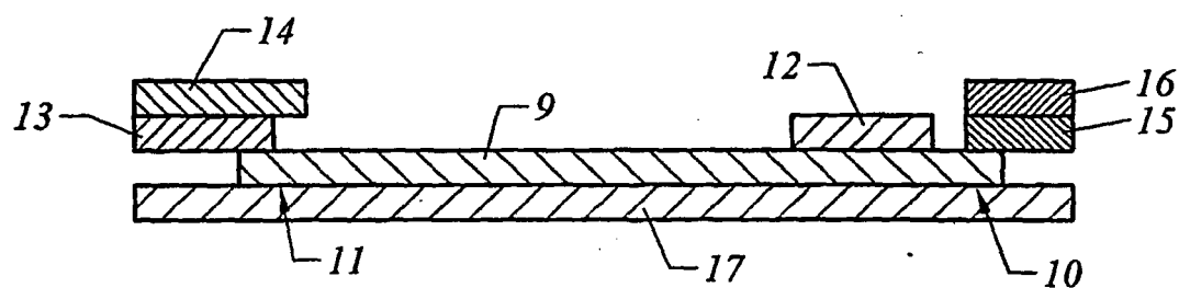
Side View of Strip with Blood Filter in Port-1
