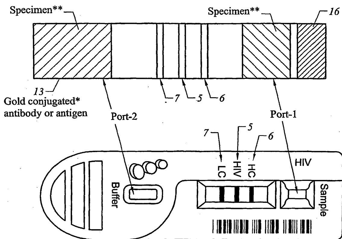
Top view of strip structure
