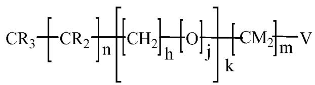
Formula I
