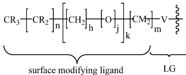
Formula IIA
