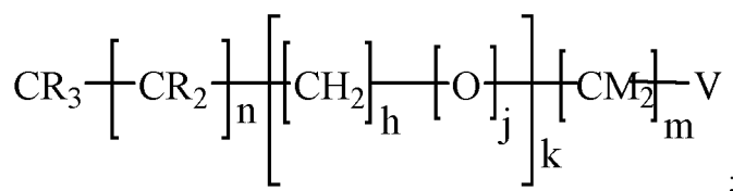
Formula I
