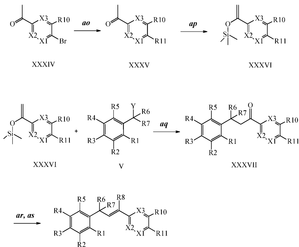
Scheme XXXI
