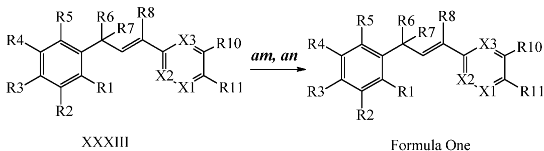
Scheme XXX
