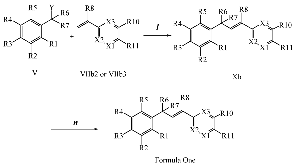
Scheme VIII
