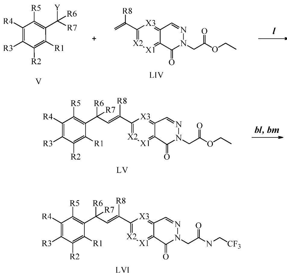
Scheme XXXIX
