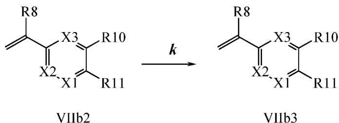
Scheme V
