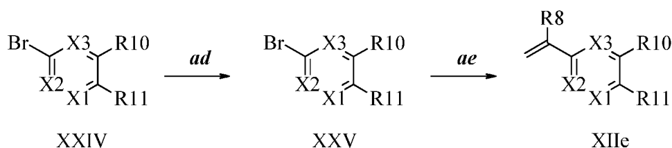
Scheme XVIII
