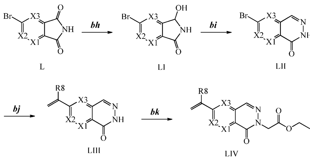
Scheme XXXVIII
