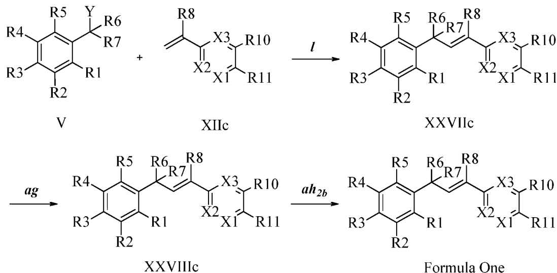
Scheme XXII
