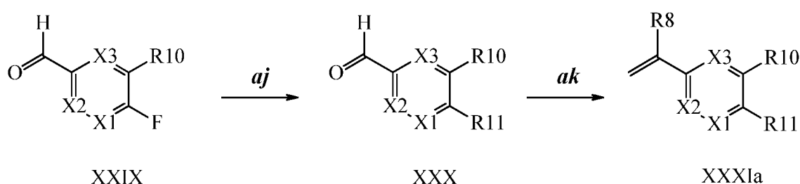
Scheme XXVII
