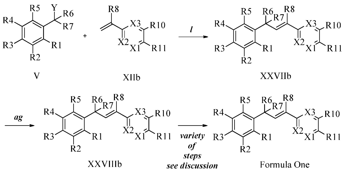
Scheme XXI
