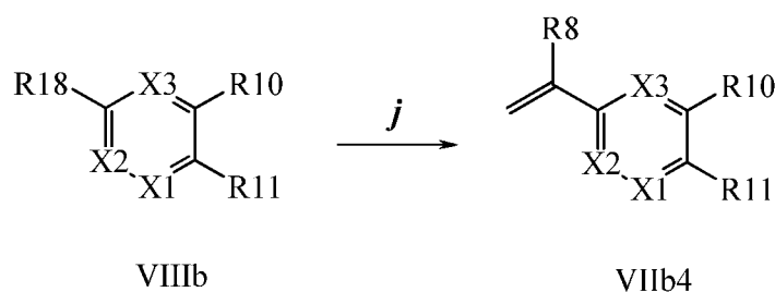
Scheme IX
