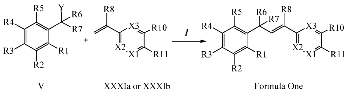
Scheme XXIX
