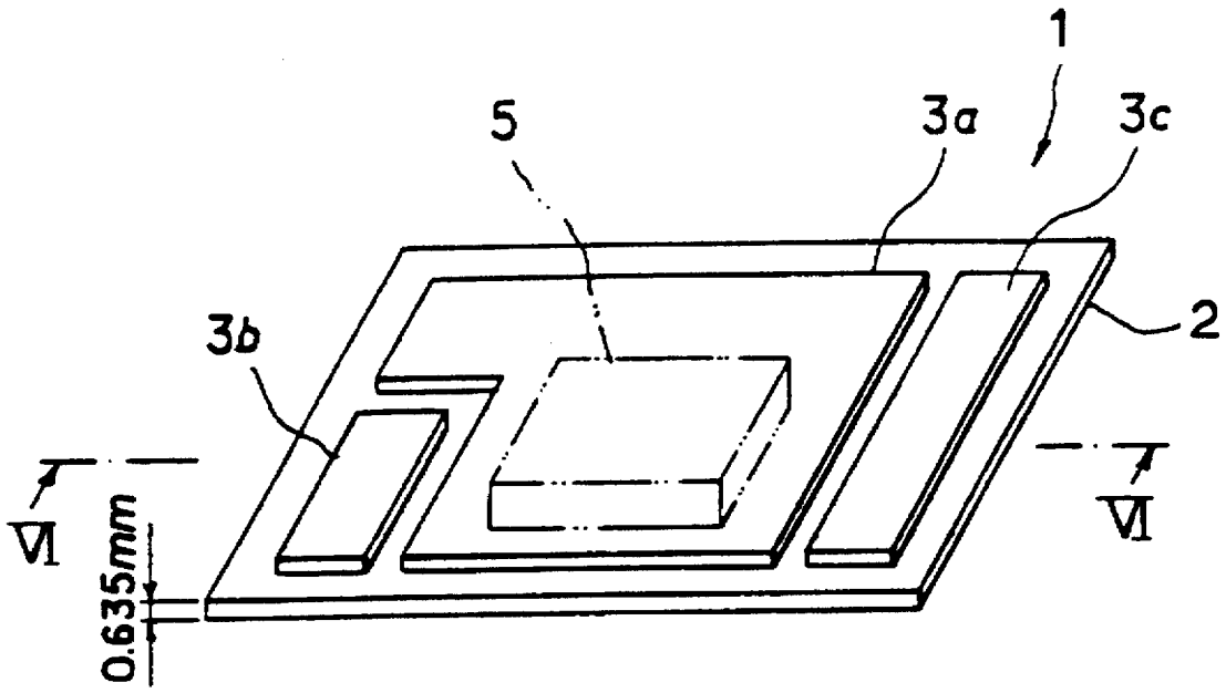
FIG. 5 PRIOR ART
