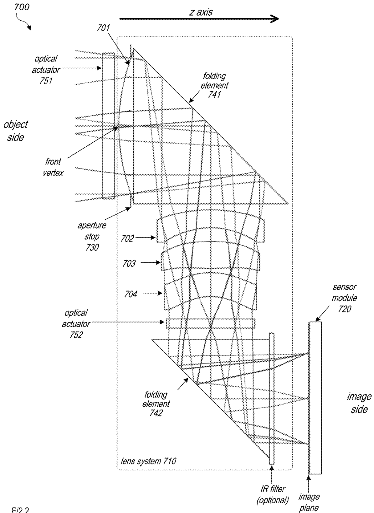
F/2.2 35mm Equivalent Focal Length: 85 mm Two solid-state autofocus optical actuators
