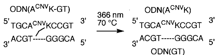
Scheme 9
