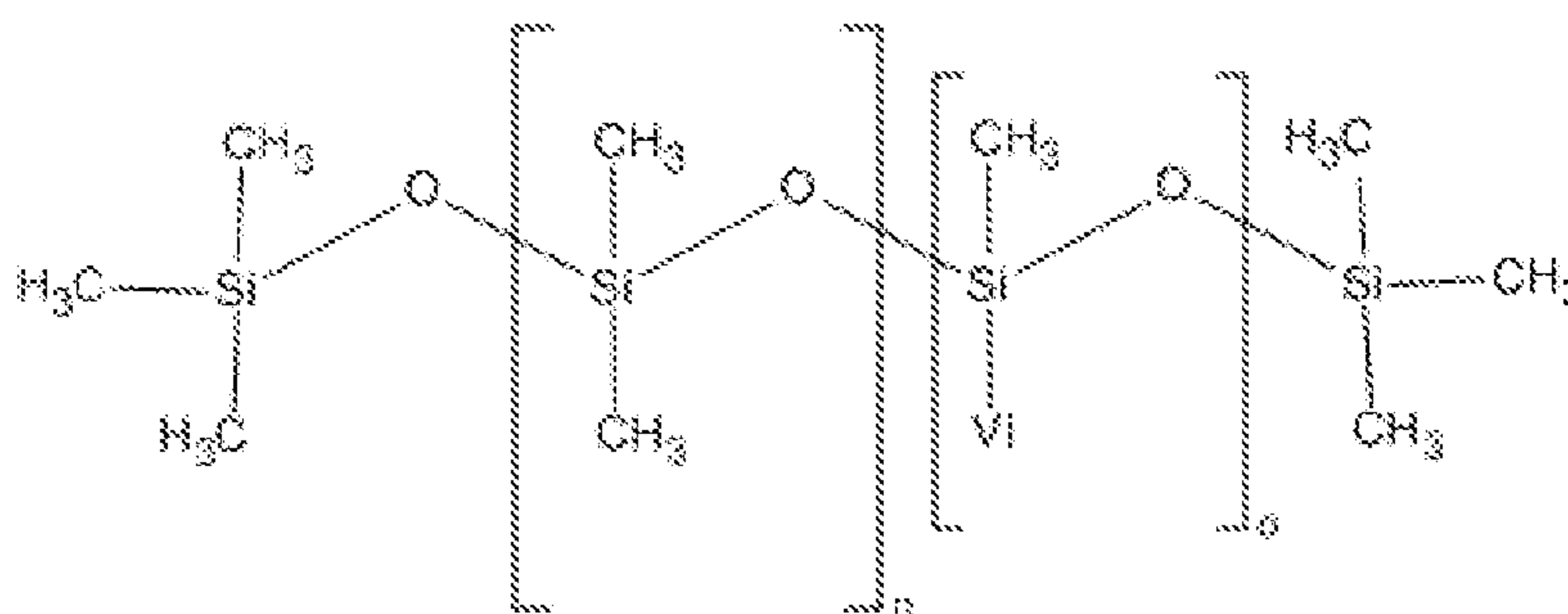
Formula I-6
