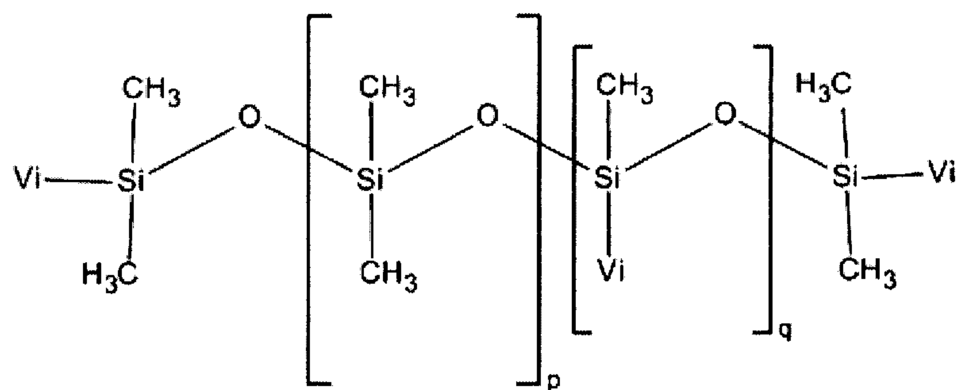
(Formula I-7)
