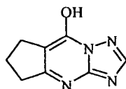
Triazaindolisine-04:
