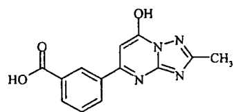
Triazaindolisine-10:
