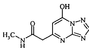
Triazaindolisine-18:
