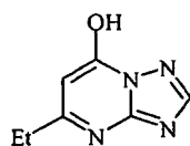
Triazaindolisine-14:
