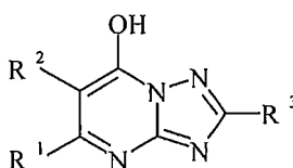
(Formel I)
