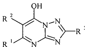
(Formule I)
