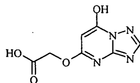
Triazaindolisine-13:
