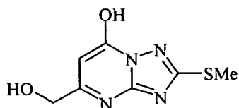
Triazaindolisine-15:
