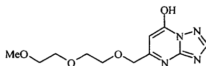
Triazaindolisine-17:
