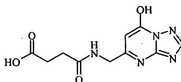
Triazaindolisine-16:
