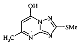
Triazaindolisine-08:
