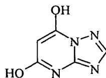
Triazaindolisine-05:
