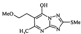
Triazaindolisine-19:
