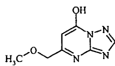
Triazaindolisine-02:
