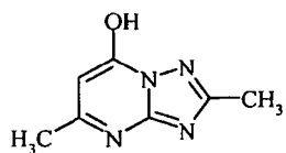
Triazaindolisine-09:
