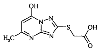
Triazaindolisine-12:
