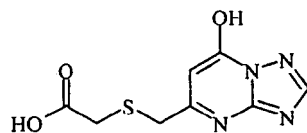
Triazaindolisine-03:
