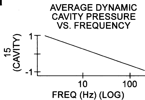
FIG. 3.01b (PRIOR ART)
