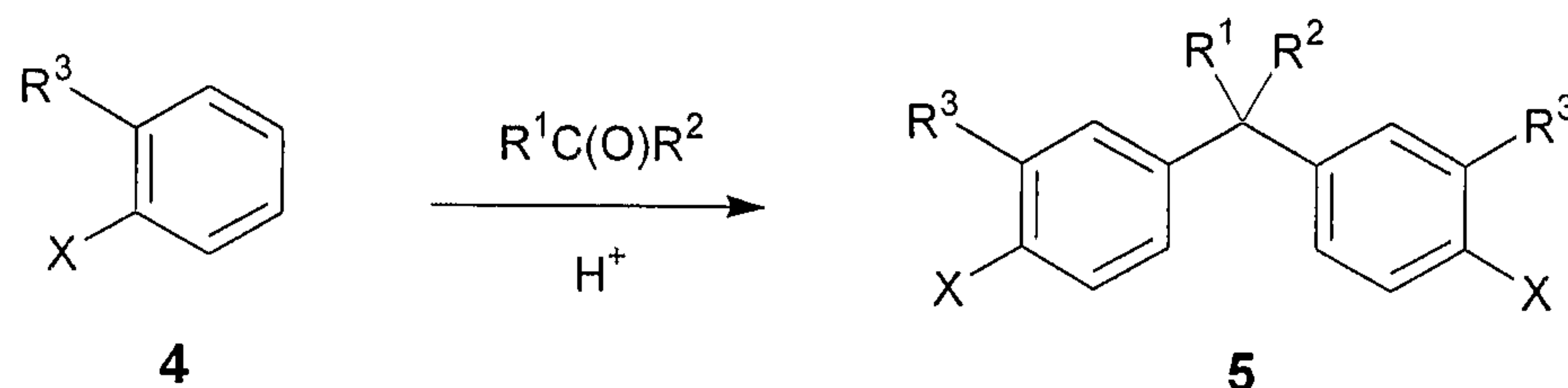
SCHEME 2
