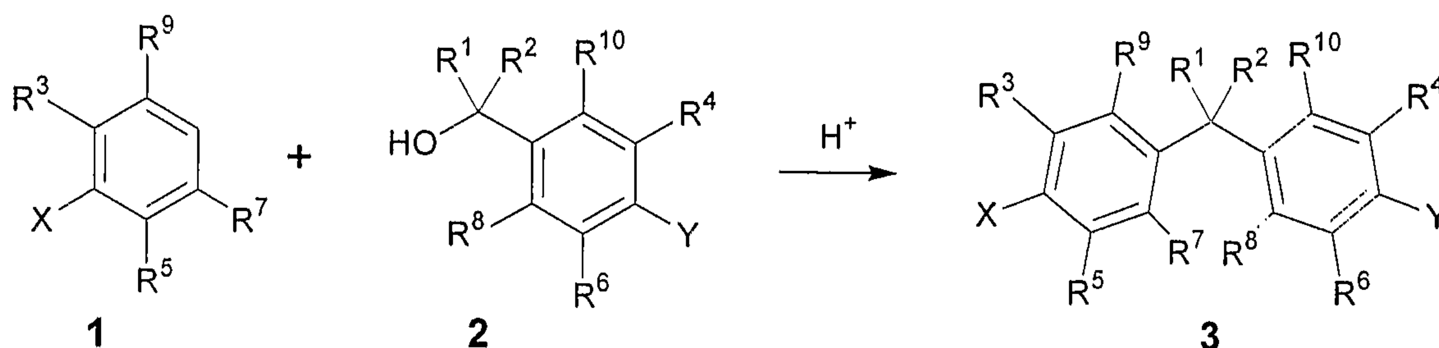
SCHEME 1
