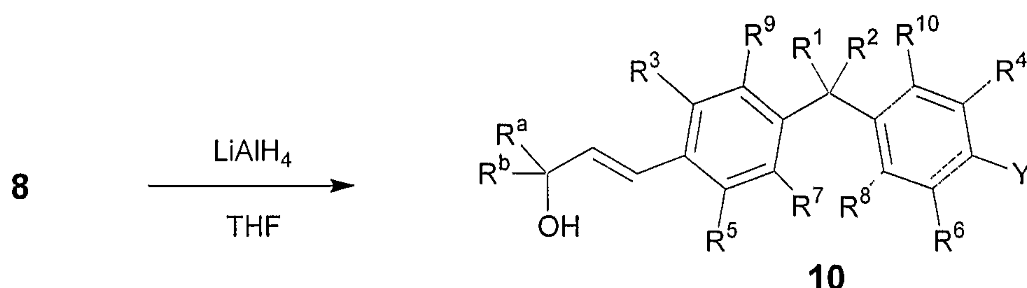
SCHEME 5
